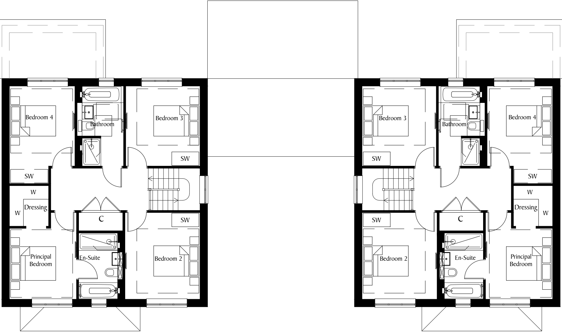
M4.15 Plot 179 M4.15 Plot 178 First Floor
