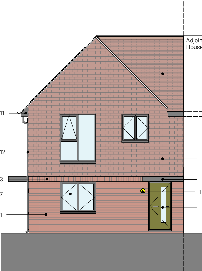
Front Elevation
