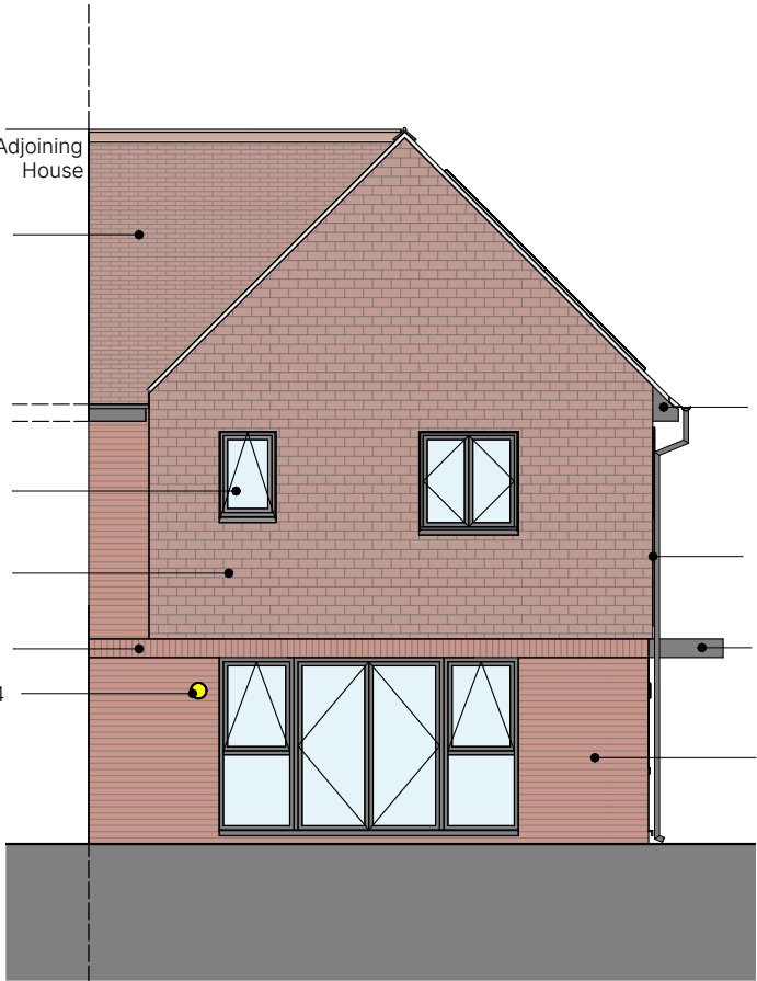
Rear Elevation
