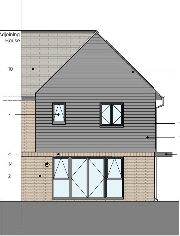
Rear Elevation 1 : 100
