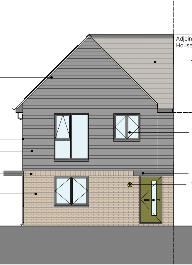
Front Elevation 1 : 100
