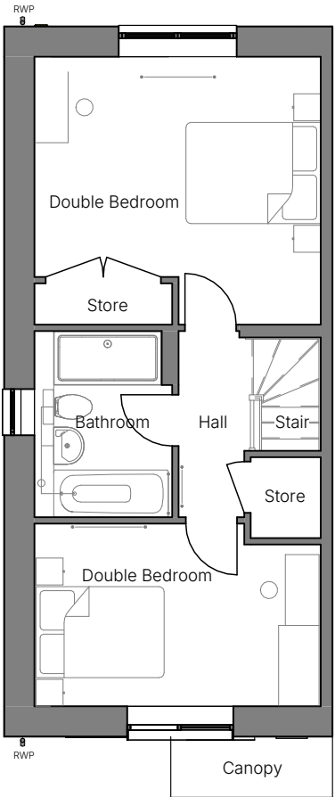
First Floor Plan 1 : 100
