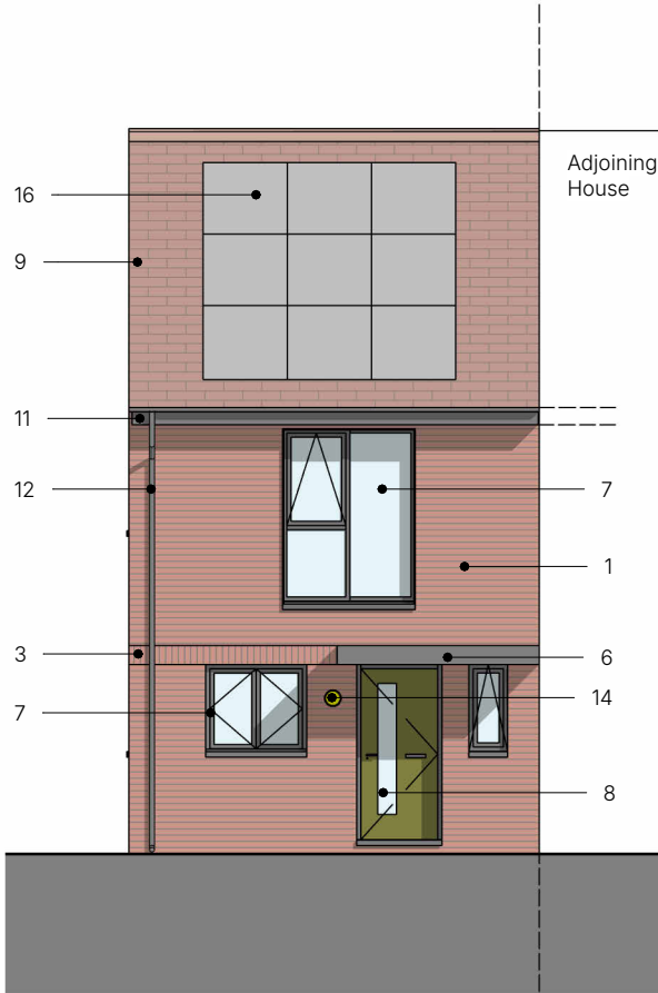
Front Elevation
