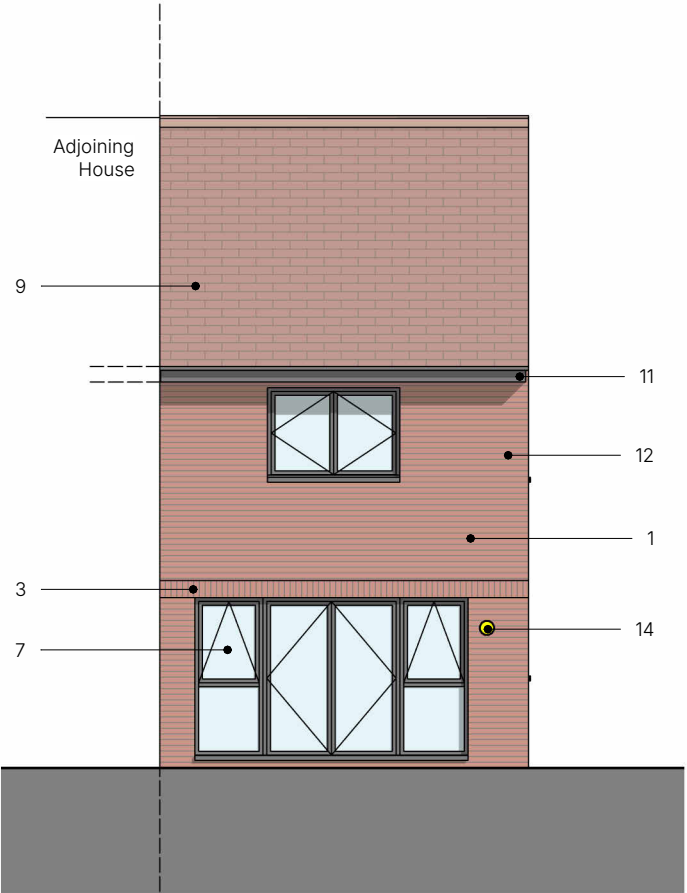
Rear Elevation
