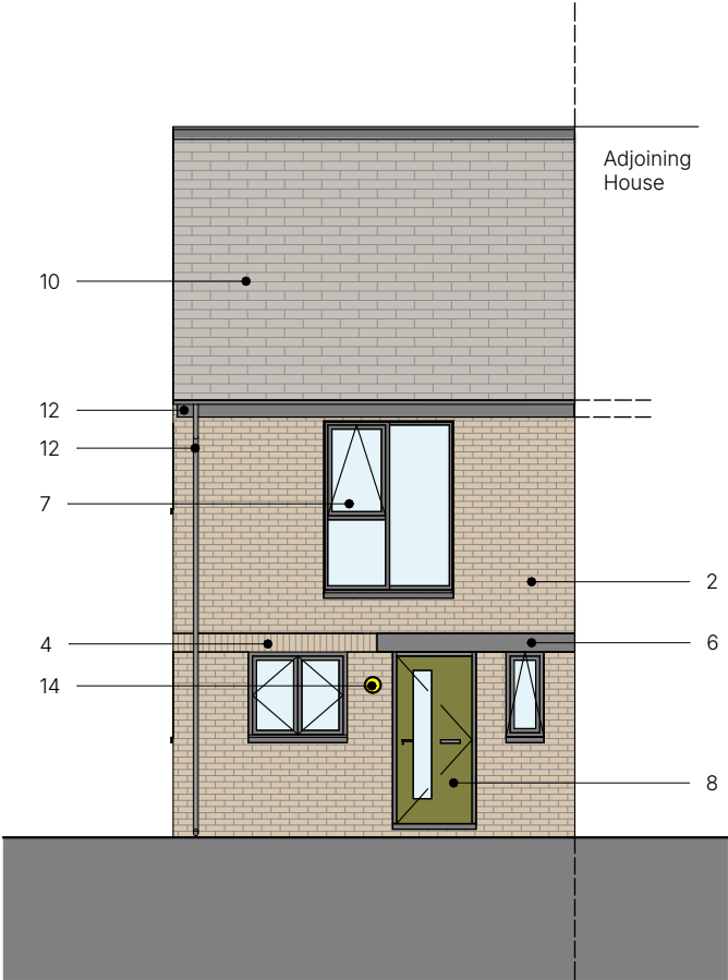
Front Elevation 1 : 100
