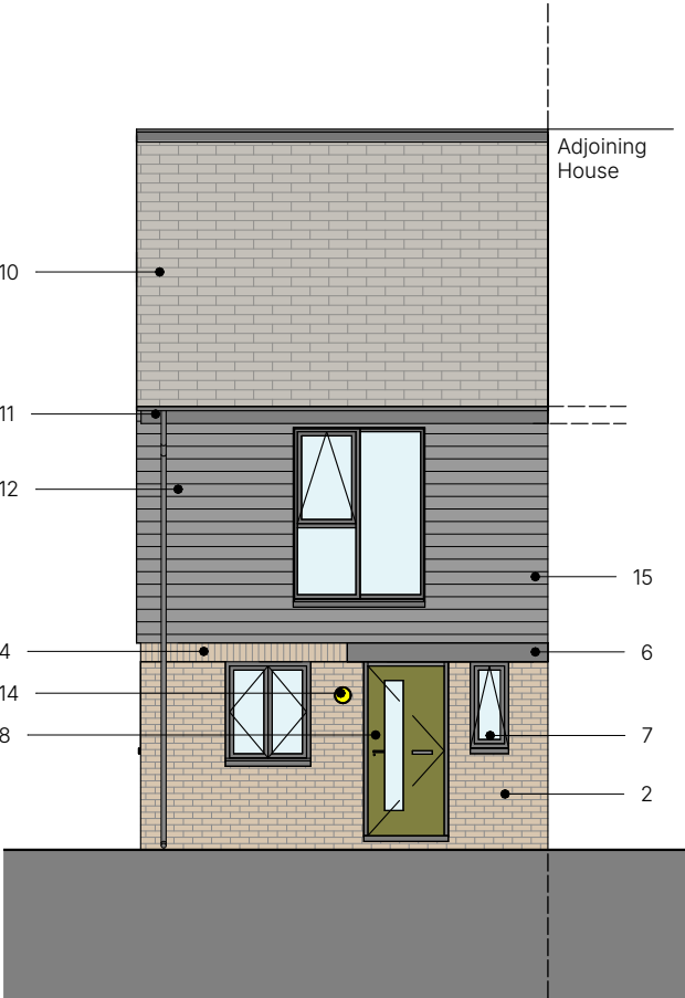
Front Elevation 1 : 100
