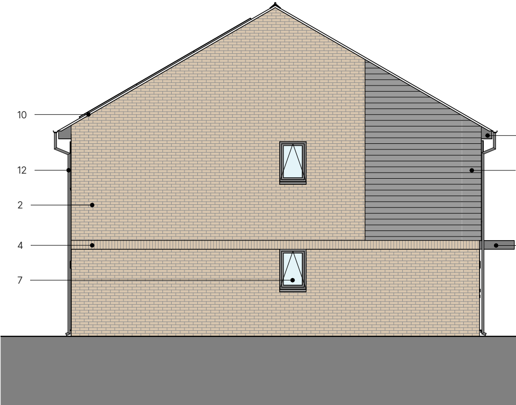
Side Elevation 1 : 100
