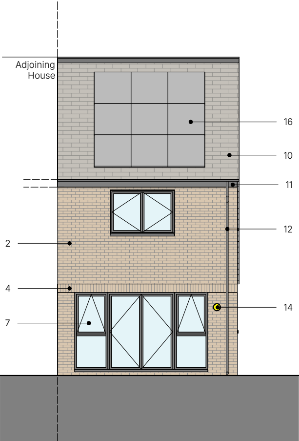
Rear Elevation 1 : 100
