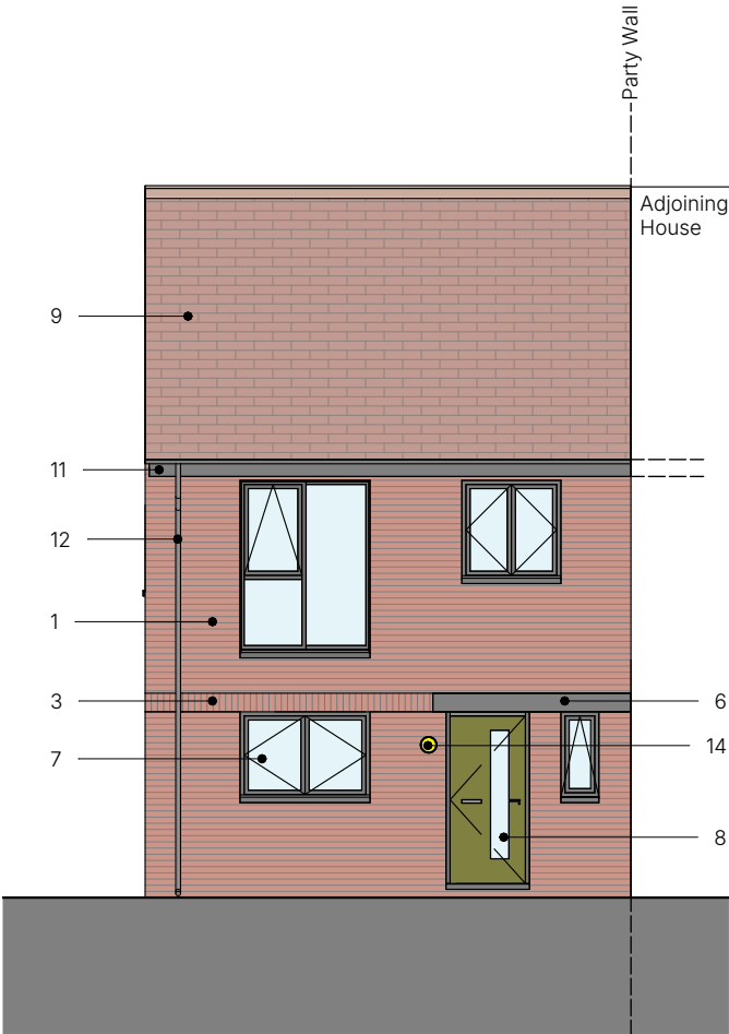
Front Elevation
