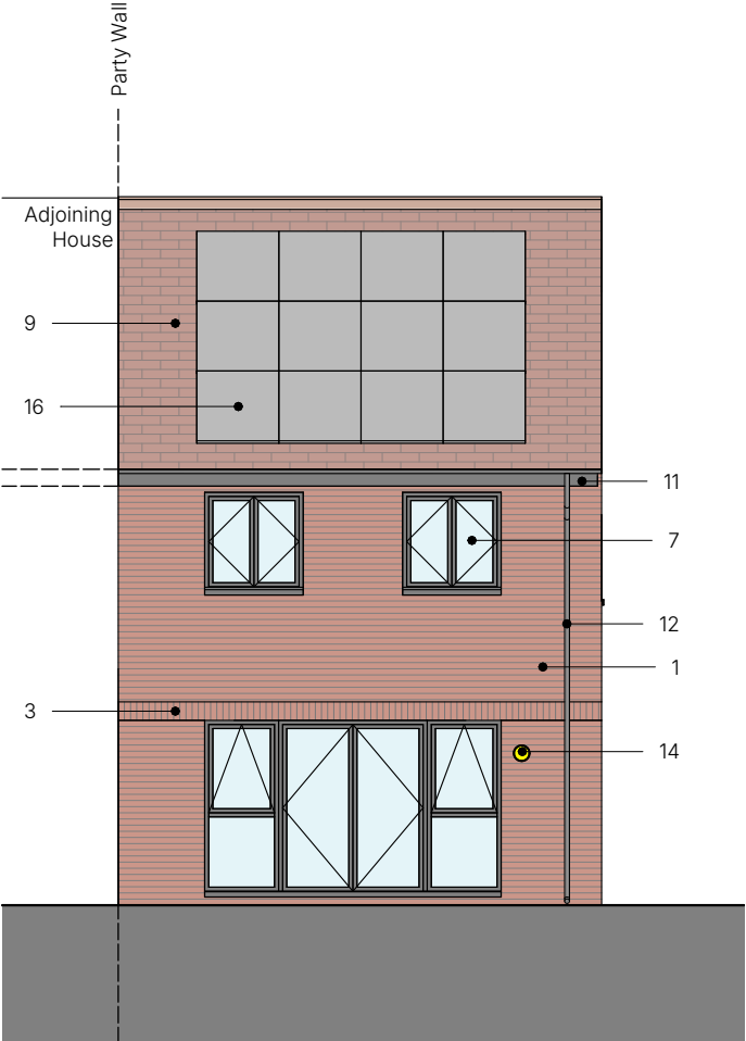
Rear Elevation
