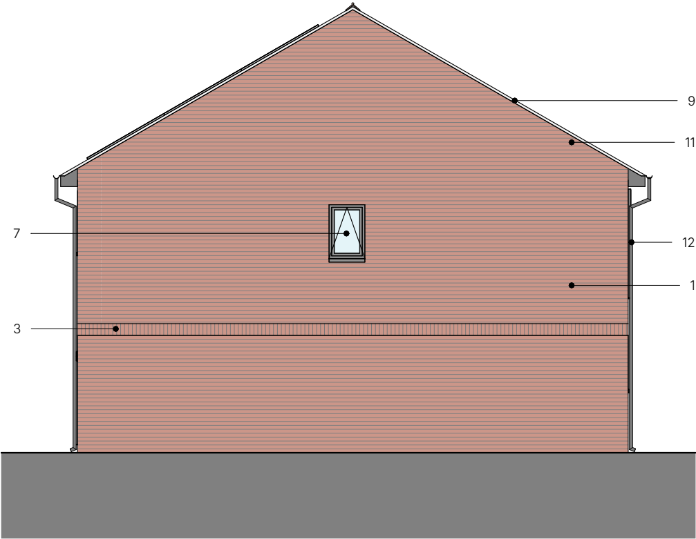
Side Elevation 1
