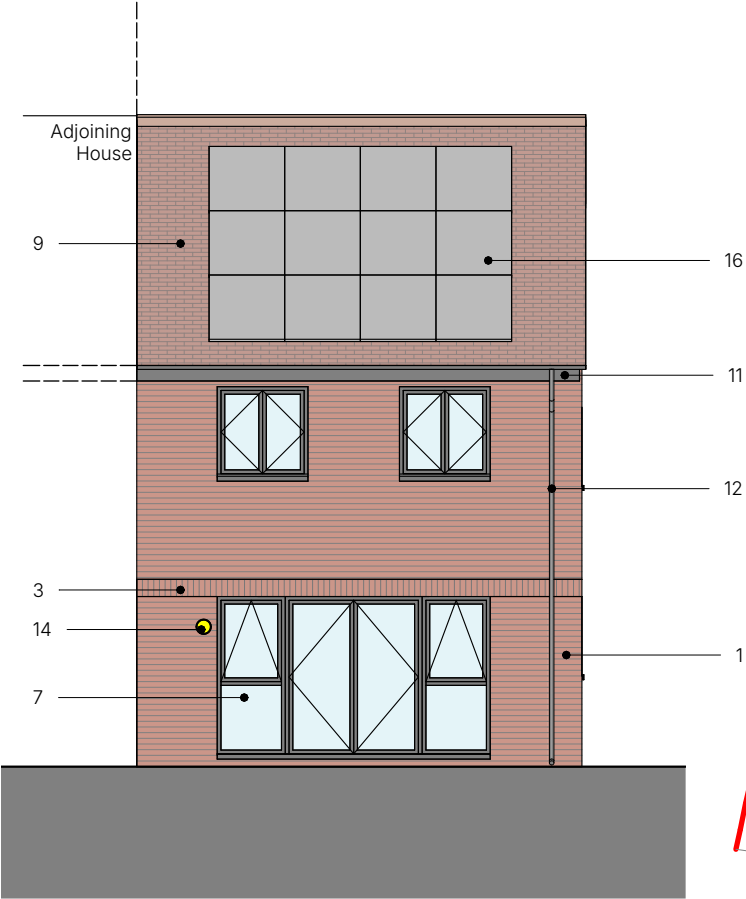
Rear Elevation 1 : 100
