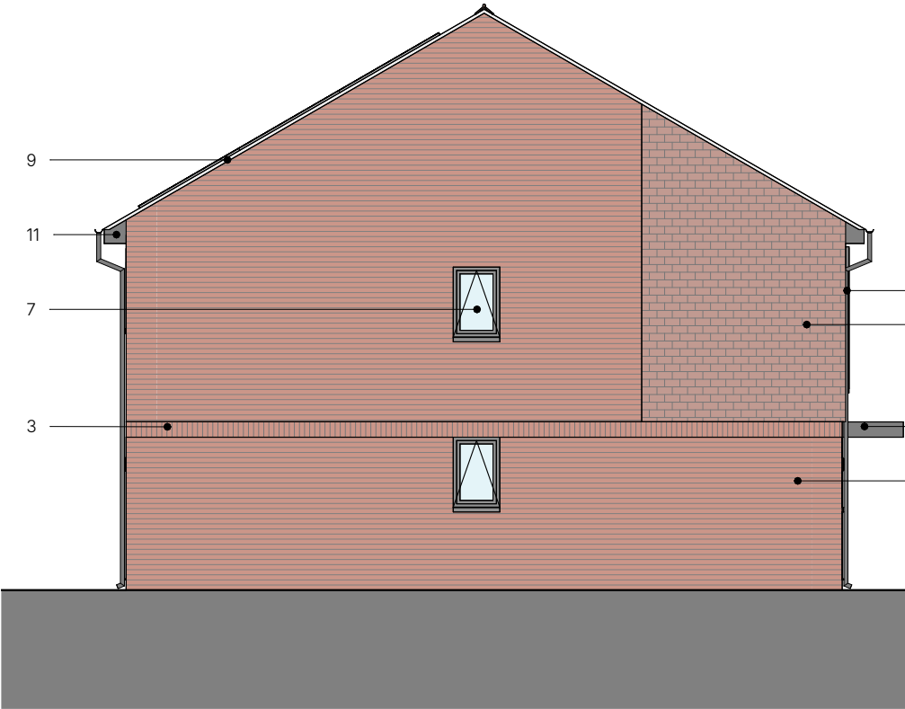
Side Elevation 1 : 100
