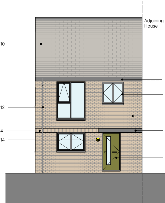
Front Elevation 1 : 100
