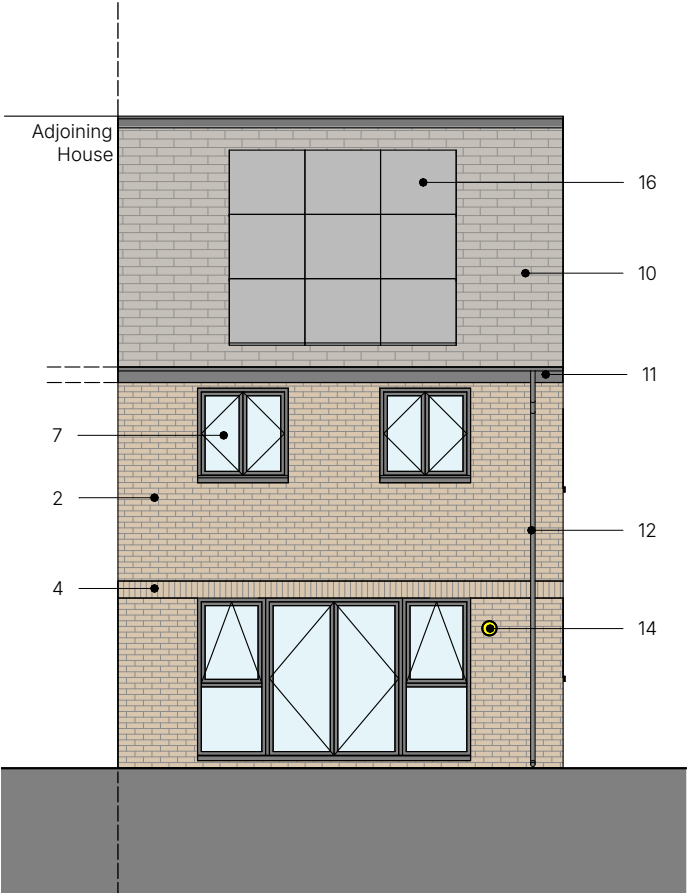
Rear Elevation 1 : 100
