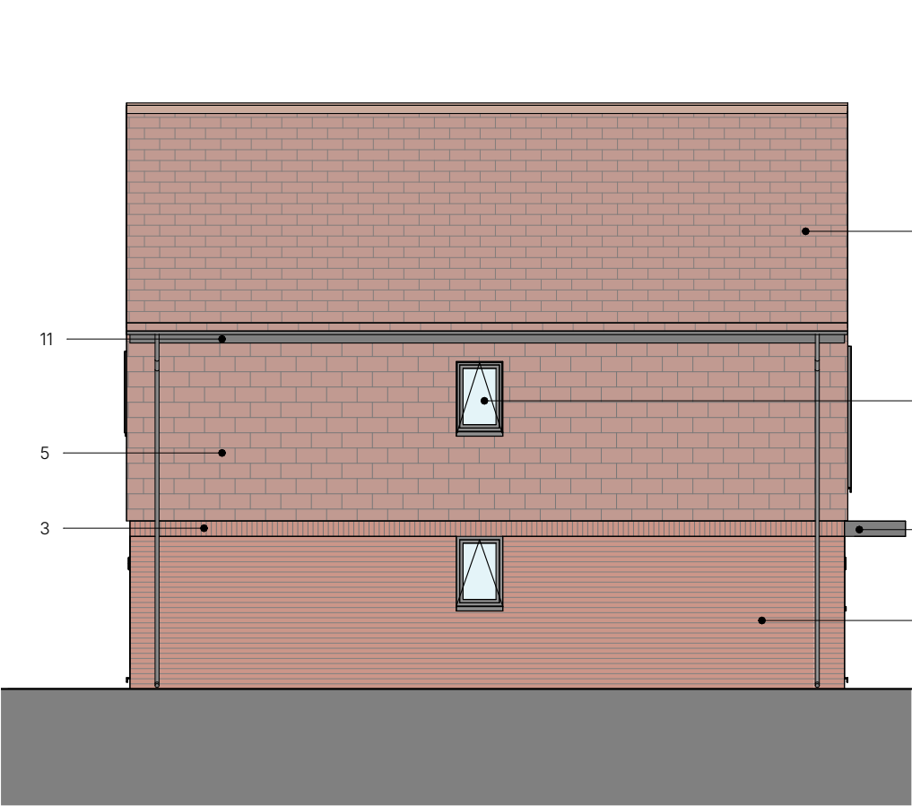
Side Elevation 1 : 100
