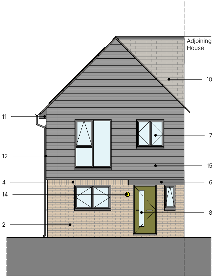
Front Elevation 1 : 100
