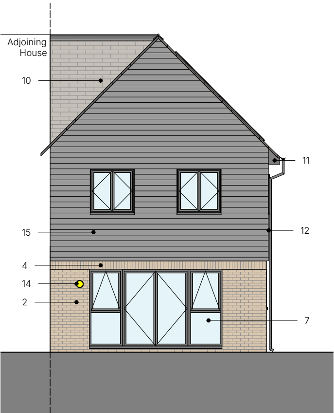
Rear Elevation 1 : 100
