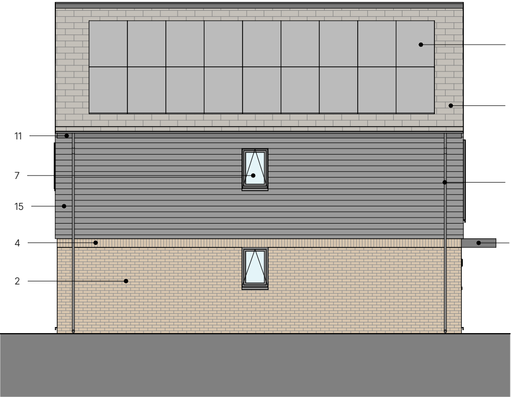
Side Elevation 1 : 100
