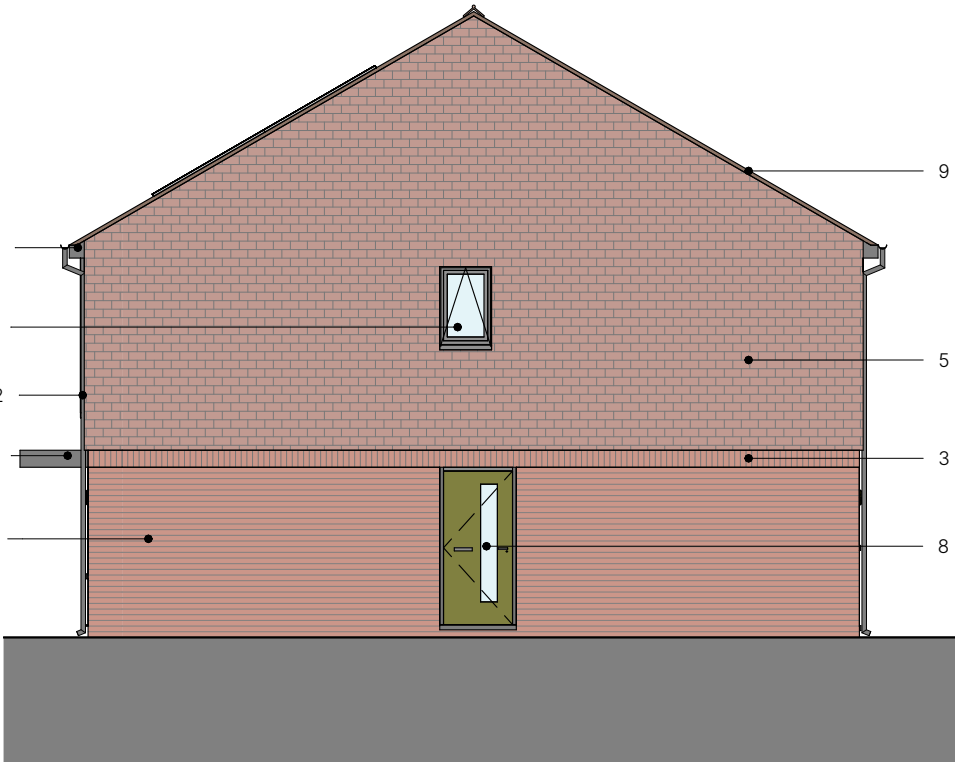
Side Elevation 2 1 : 100
