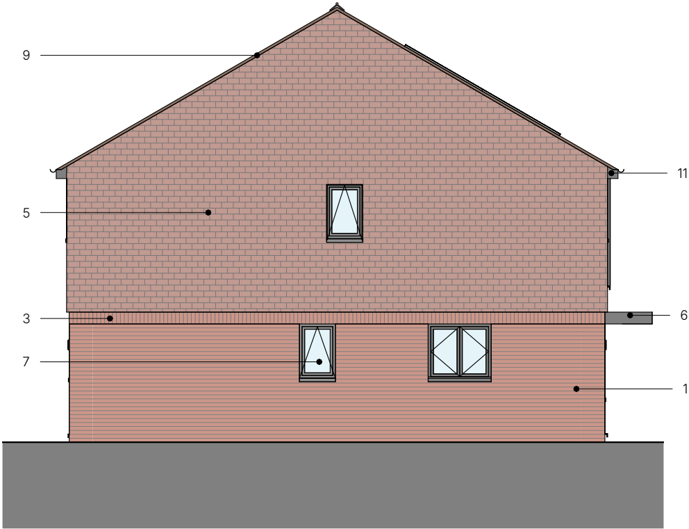
Side Elevation 1 1 : 100
