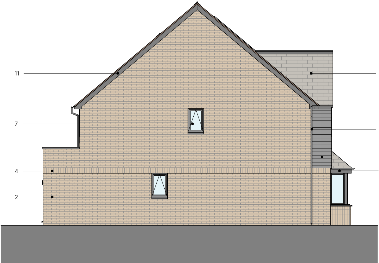
Side Elevation 2
