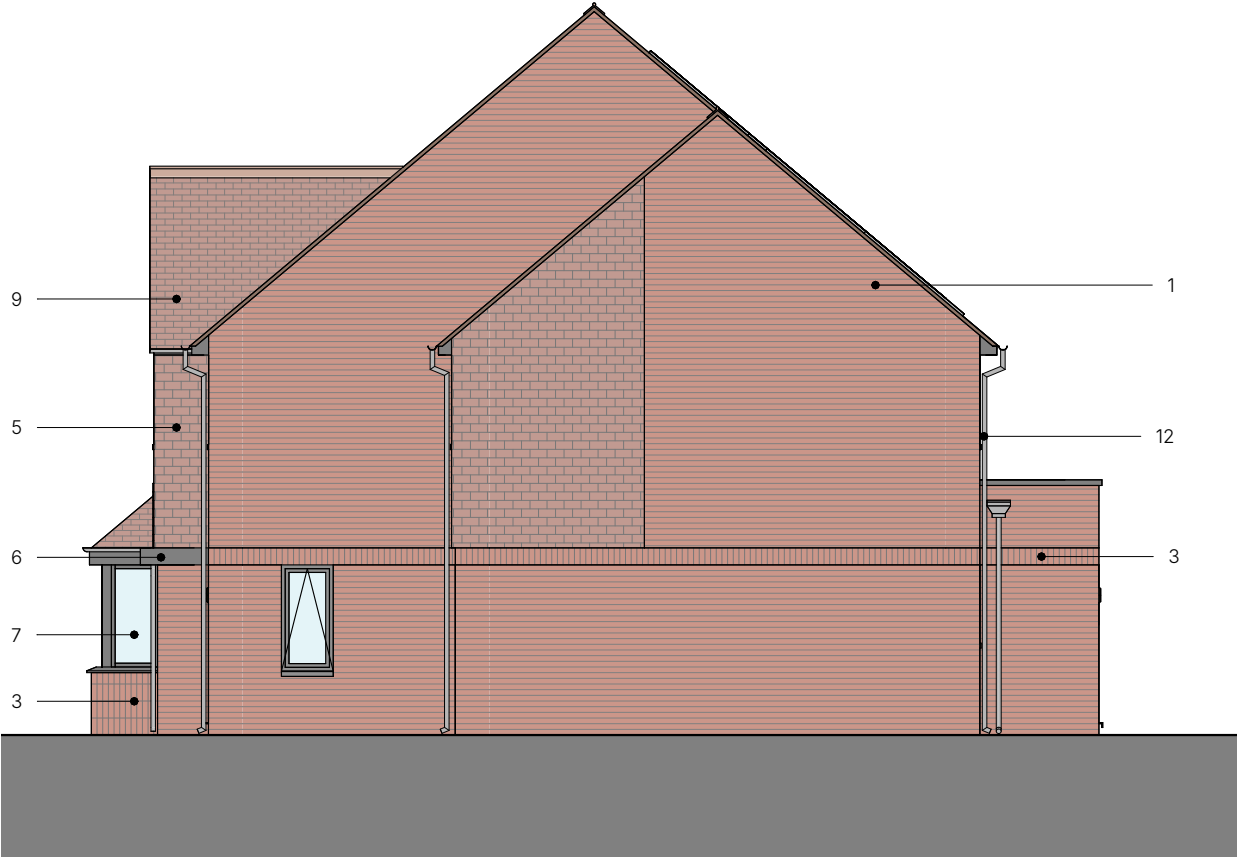
Side Elevation 1 1 : 100
