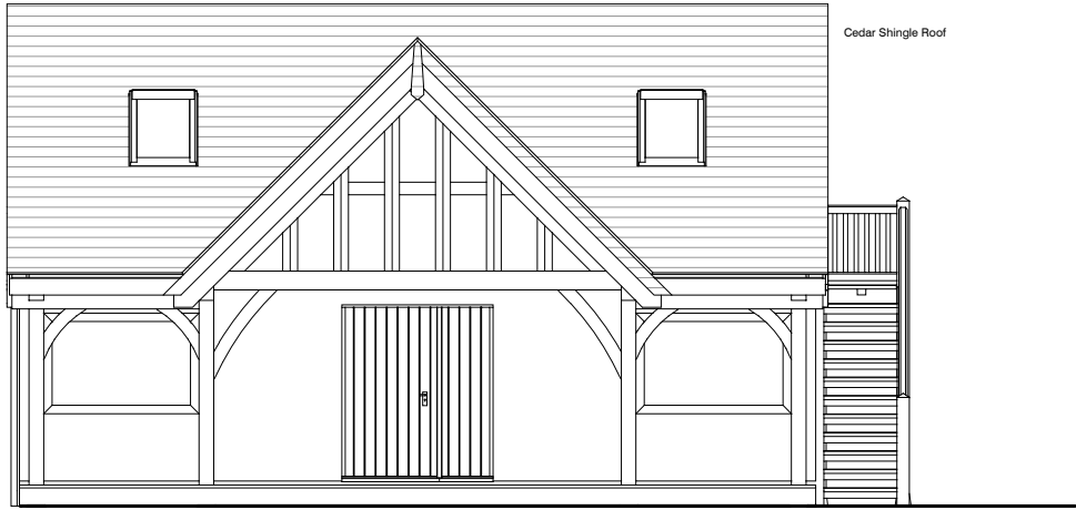
Front Elevation (North)
