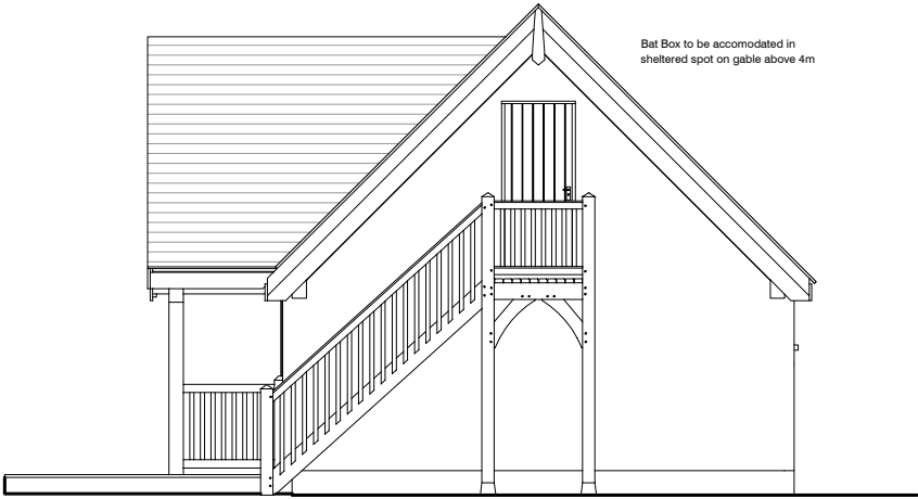
Side Elevation (West)
