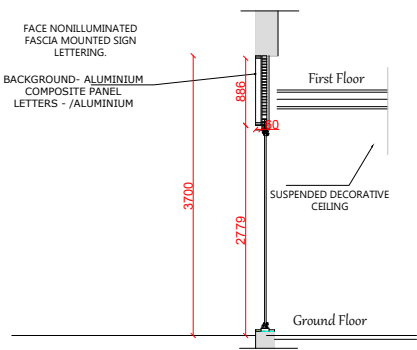
PROPOSED SIGN SECTION A-A
