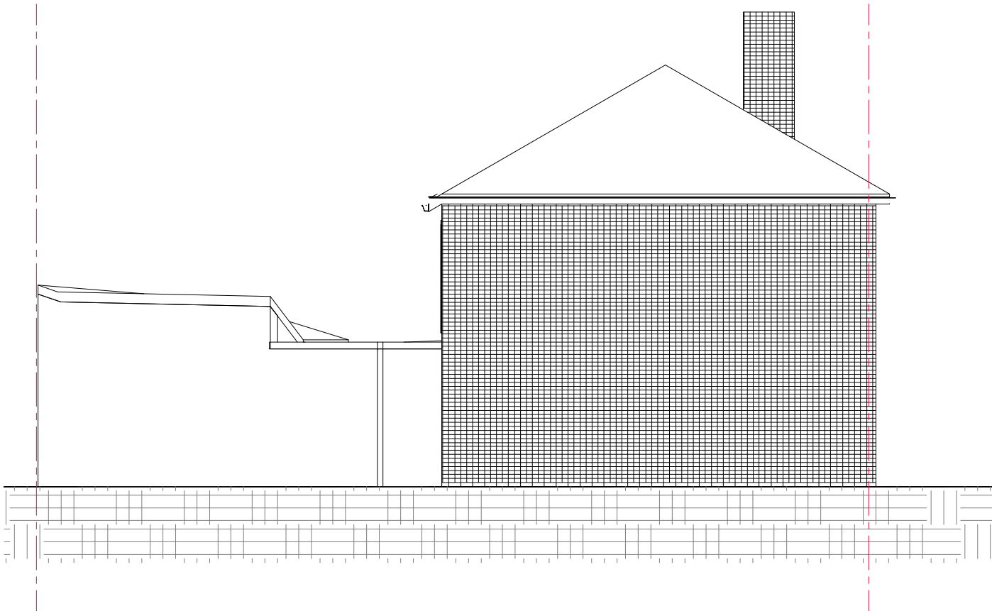
Proposed Side Elevation (South)
