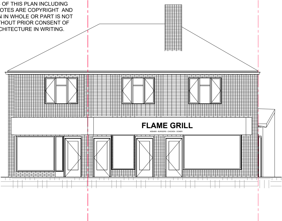
Proposed Front Elevation (East)
