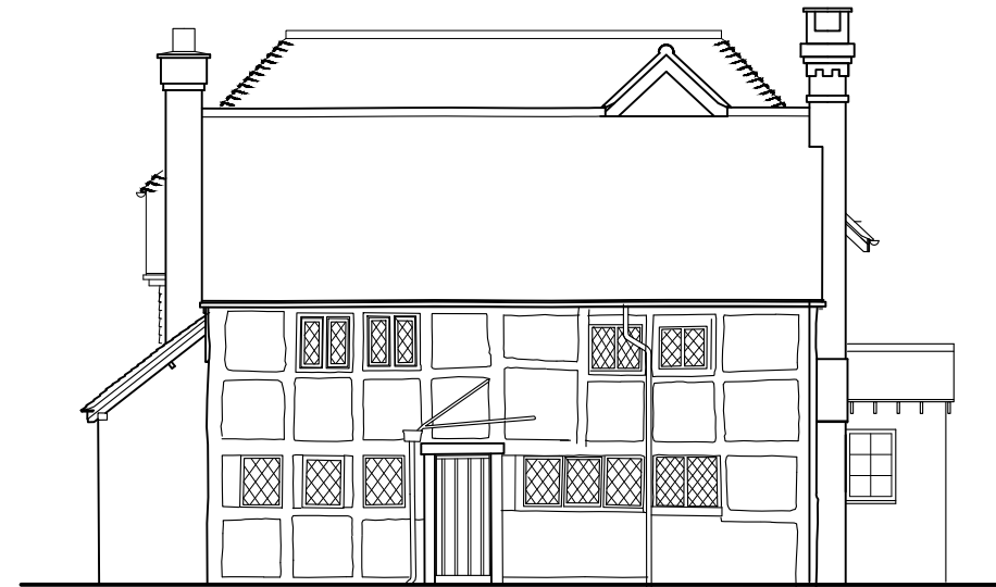
side elevation - faces west
