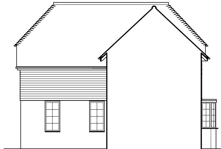
internal elevation - faces west
