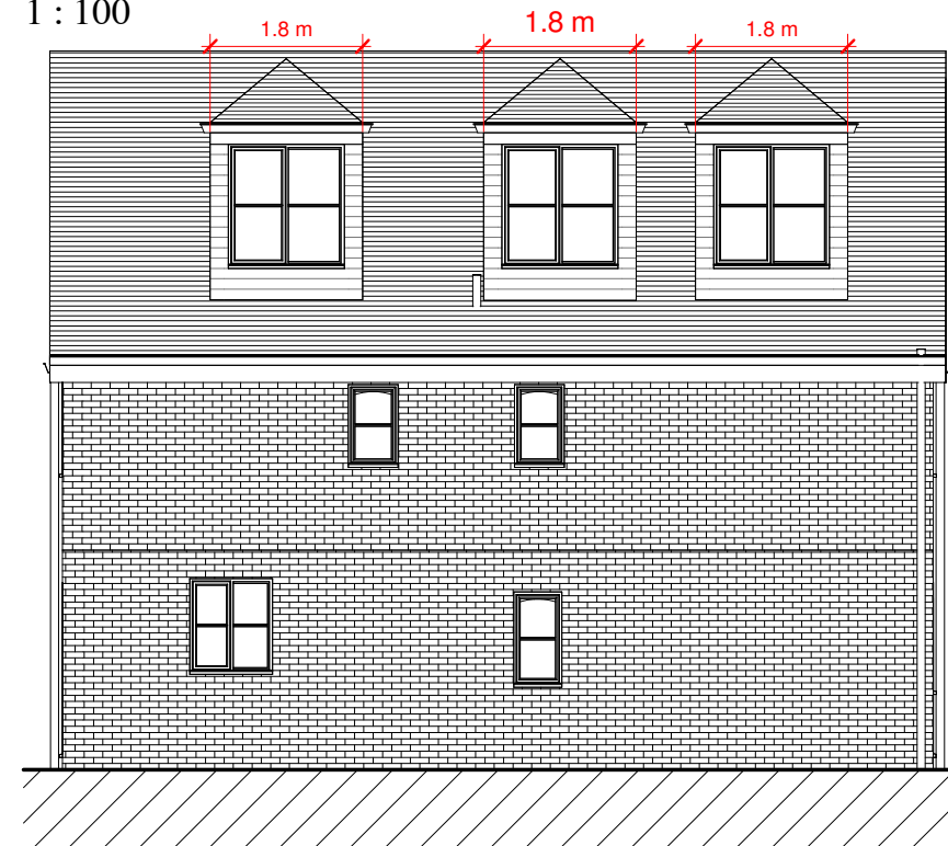
Proposed Side Elevation II 1 : 100
