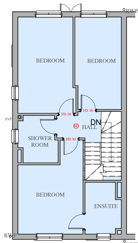
02 Proposed First Floor 1 : 100
