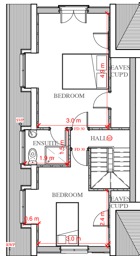
03 Proposed Second Floor 1 : 100
