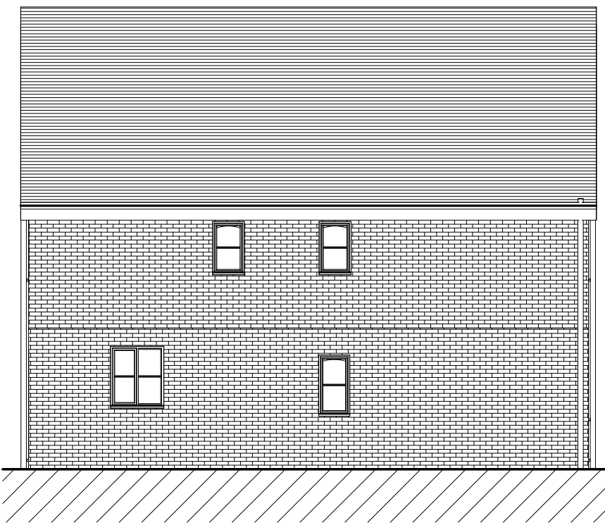
Existing Side Elevation II 1 : 100
