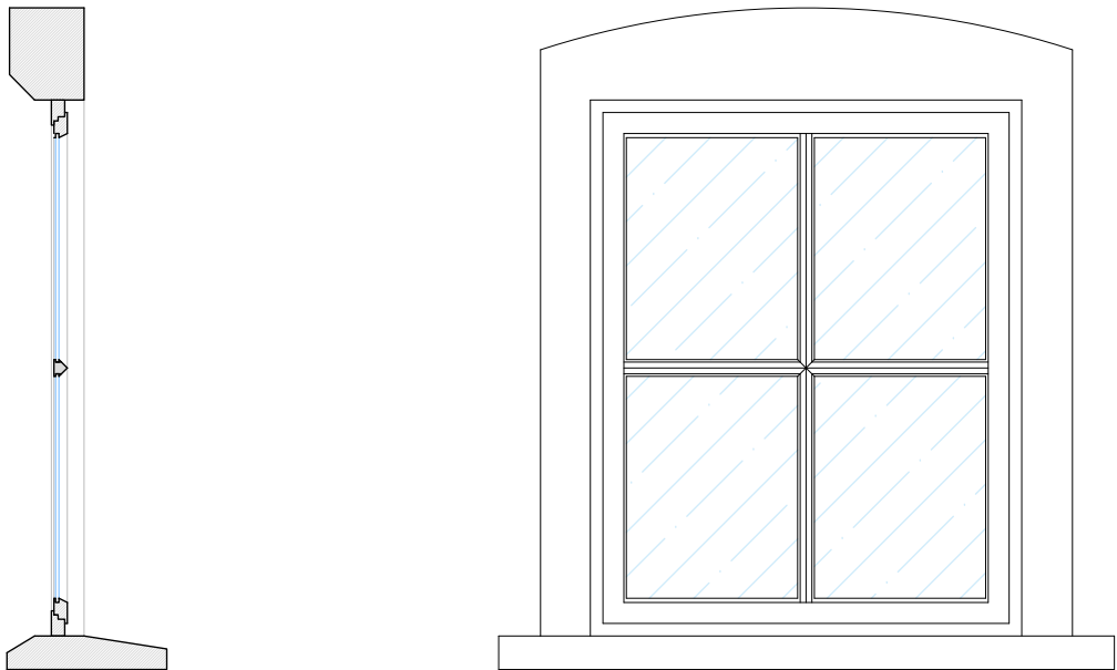
Typical Window Detail 1:10
