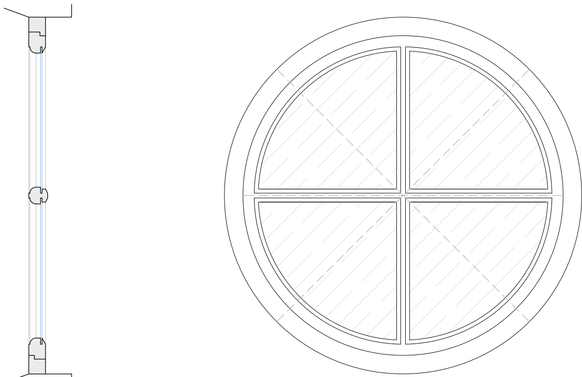
Typical Window Detail 1:10
