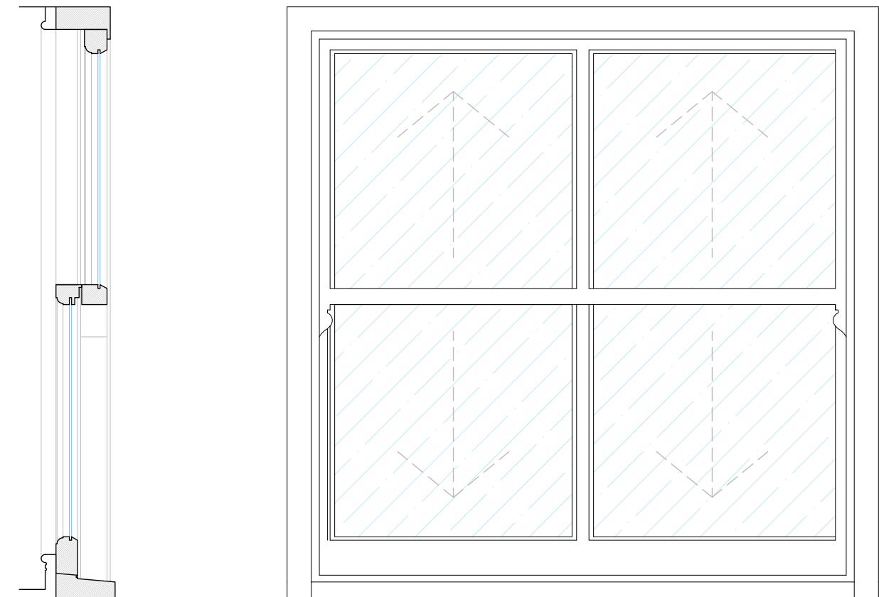
Typical Window Detail 1:10
