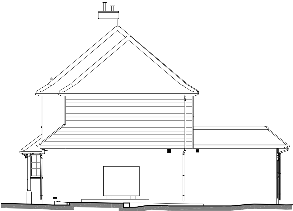
EXISTING SOUTH-EAST ELEVATION Sc. 1:100
