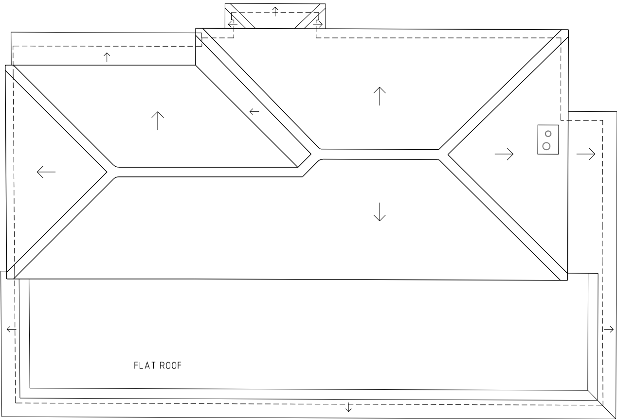
EXISTING ROOF PLAN Sc. 1:100
