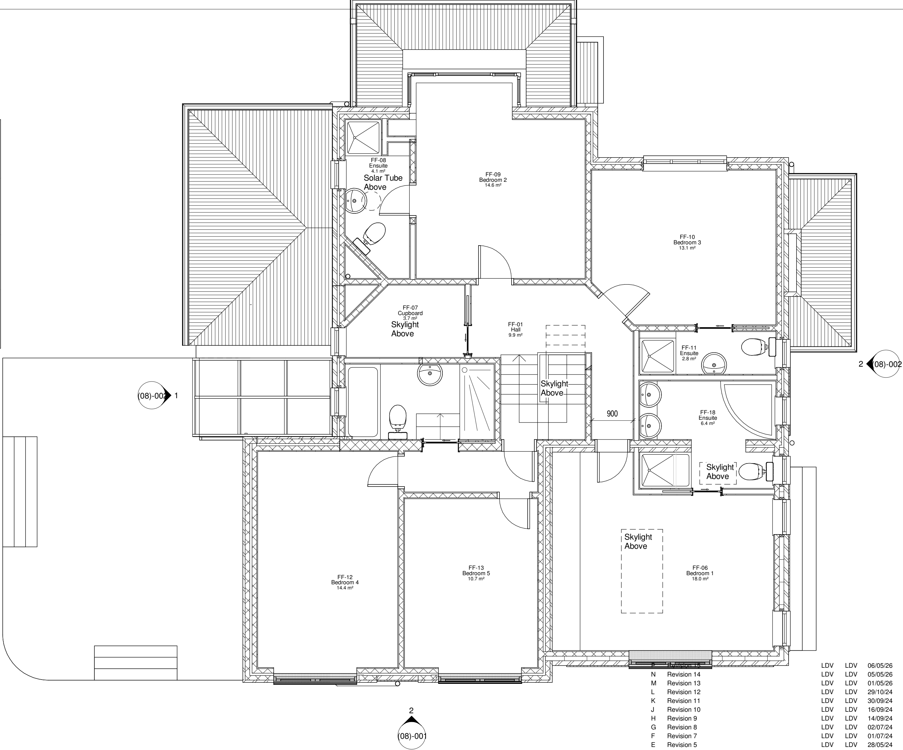
2 First Floor - Proposed Plan 1 : 50
