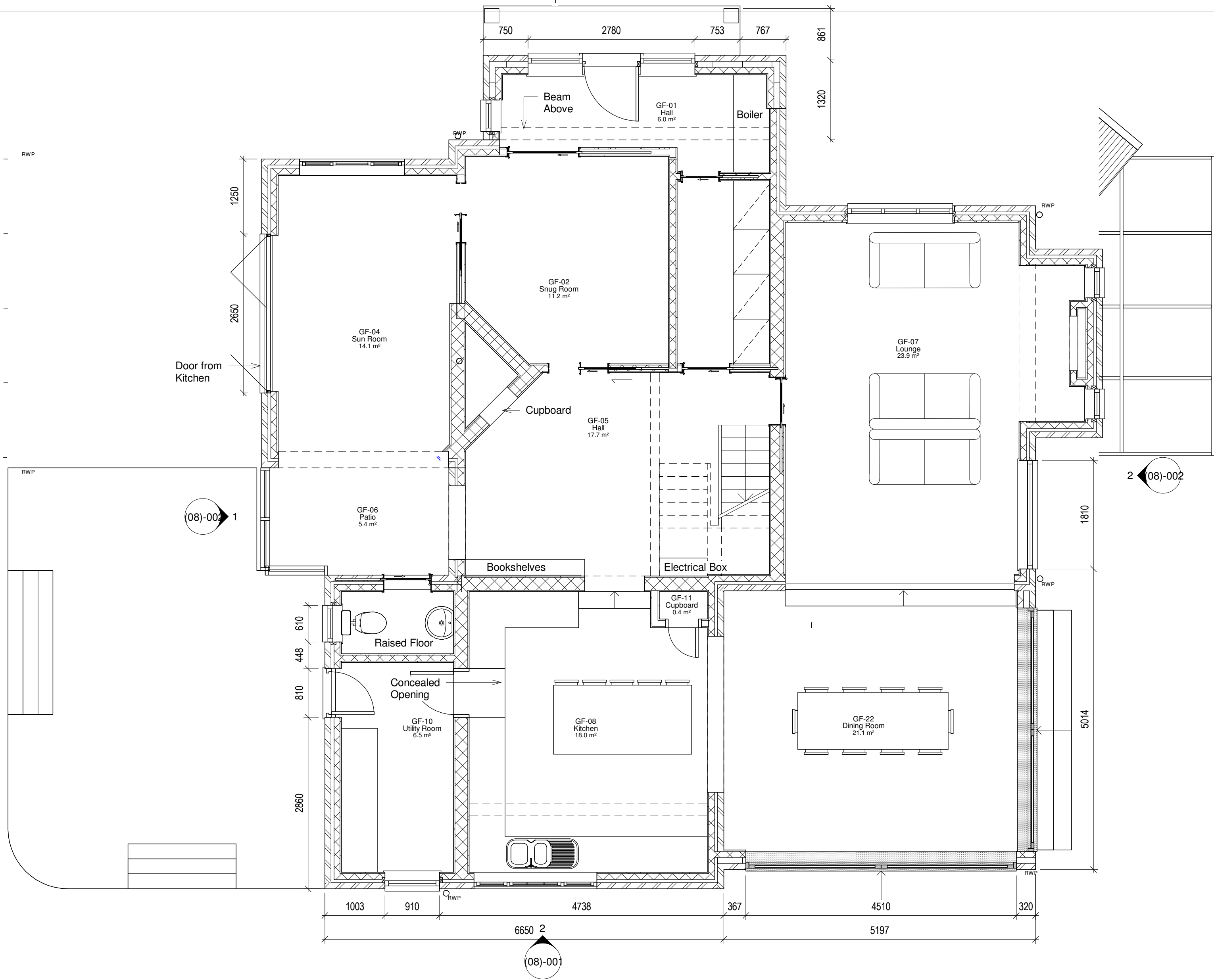
1 Ground Floor - Proposed Plan 1 : 50
