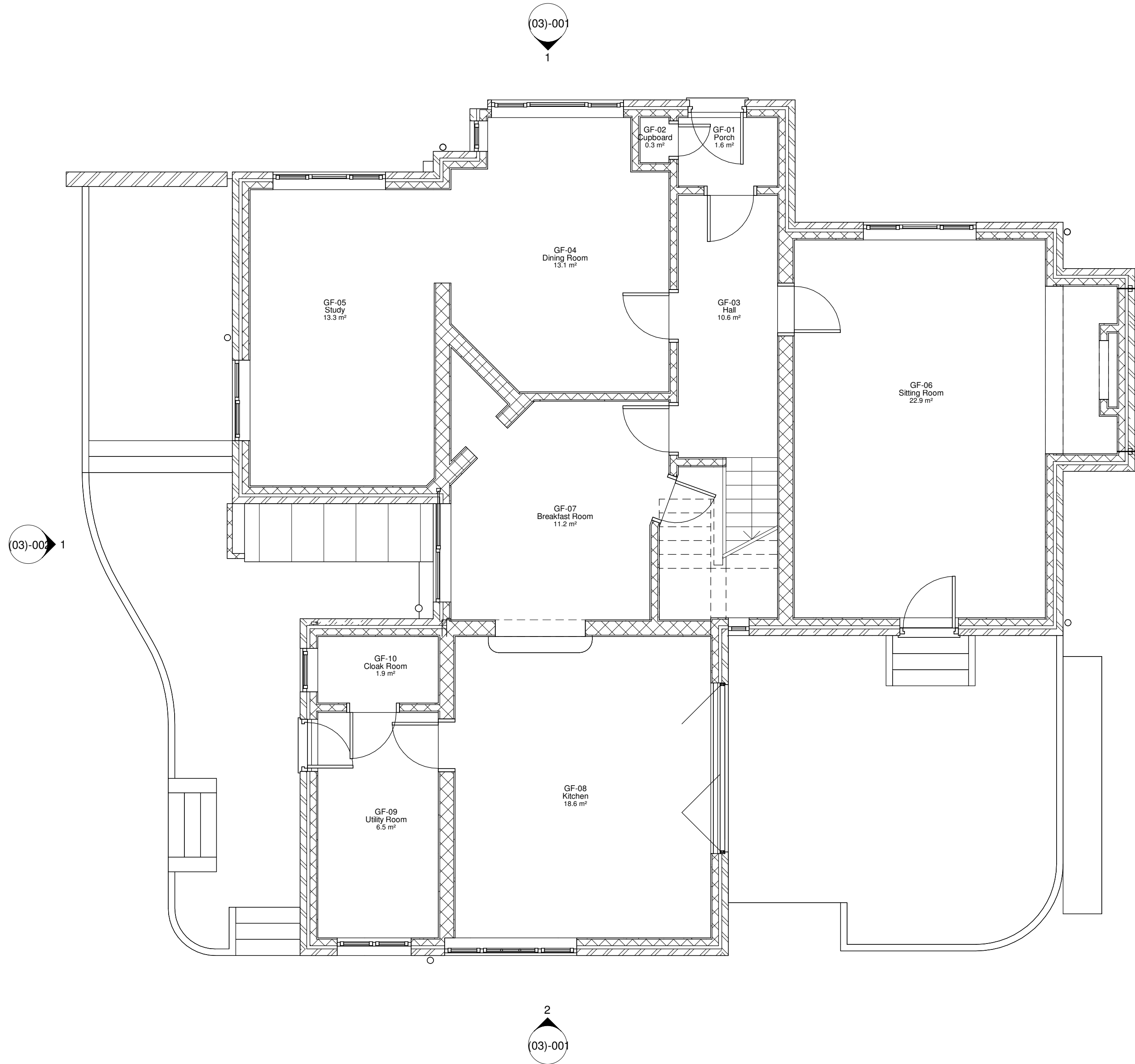
1 Ground Floor - Existing Plan 1 : 50
