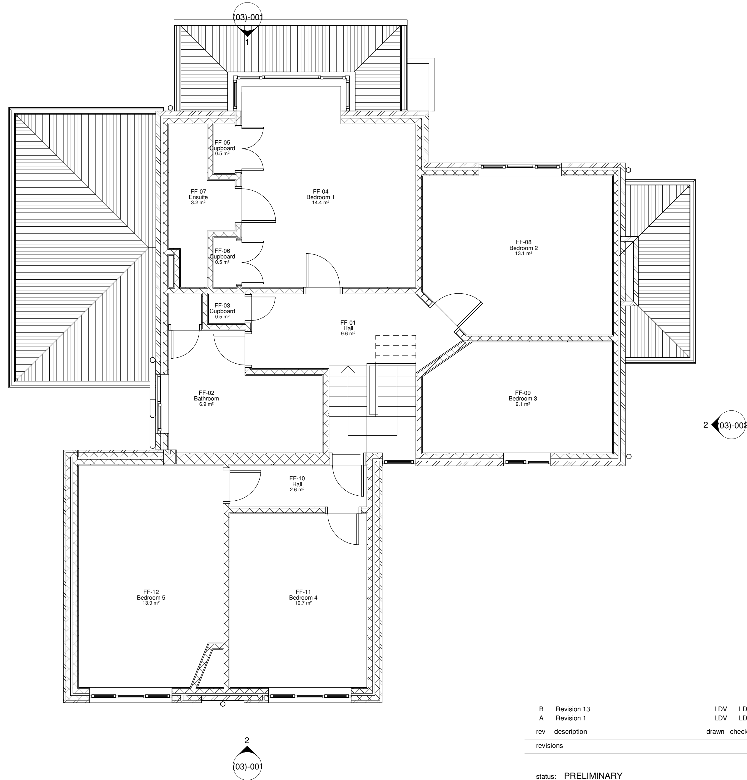
2 First Floor - Existing Plan 1 : 50
