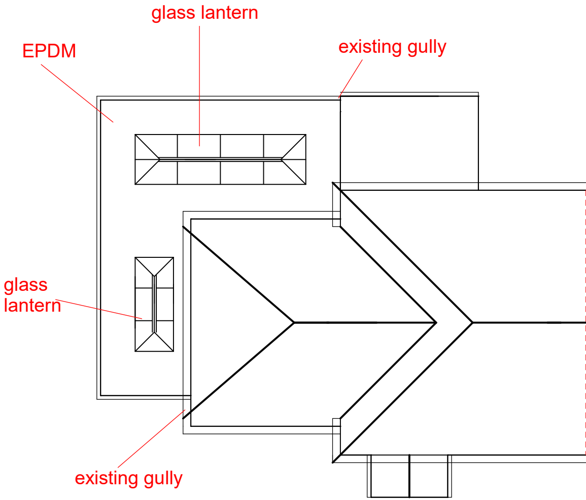
ROOF PLAN
