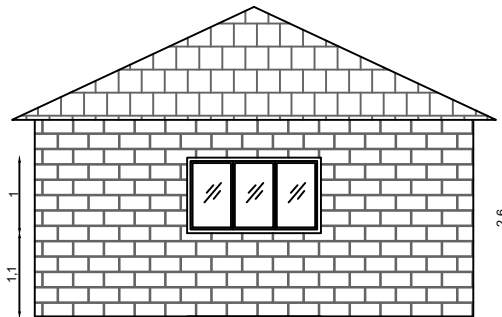
EXISTING RIGHT SIDE ELEVATION Scale 1: 100
