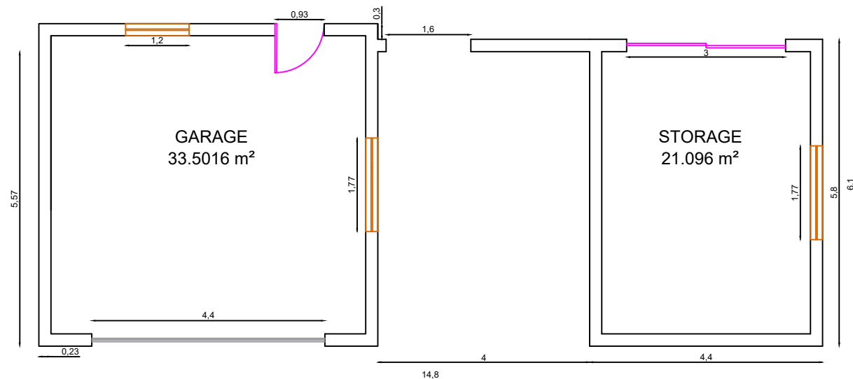
EXISTING PLAN
