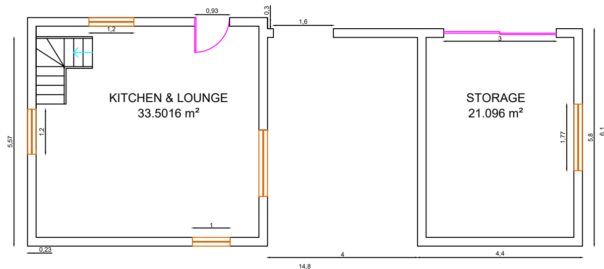
PROPOSED PLAN
