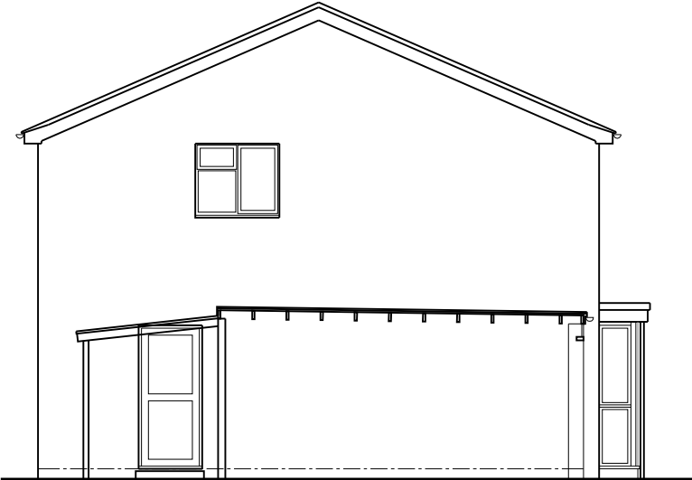
Existing Section 1:100
