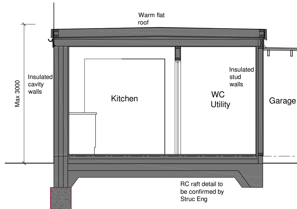
Proposed Section 1:50
