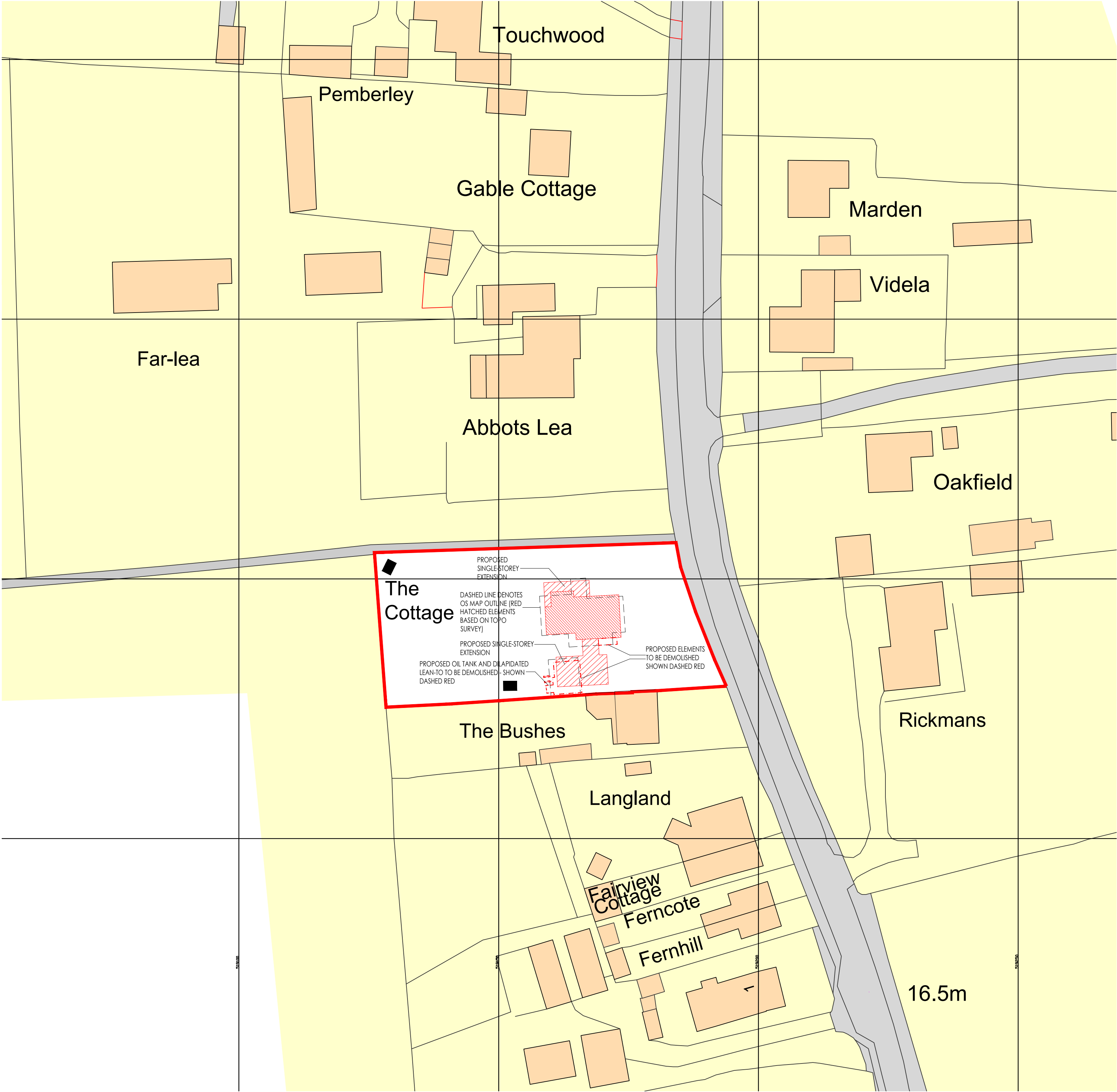
SITE BLOCK PLAN - AS PROPOSED SCALE @ 1:500 ON AN A1 SHEET
