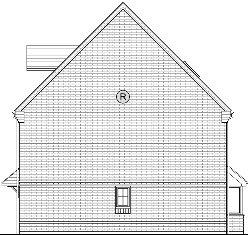
SIDE ELEVATION
