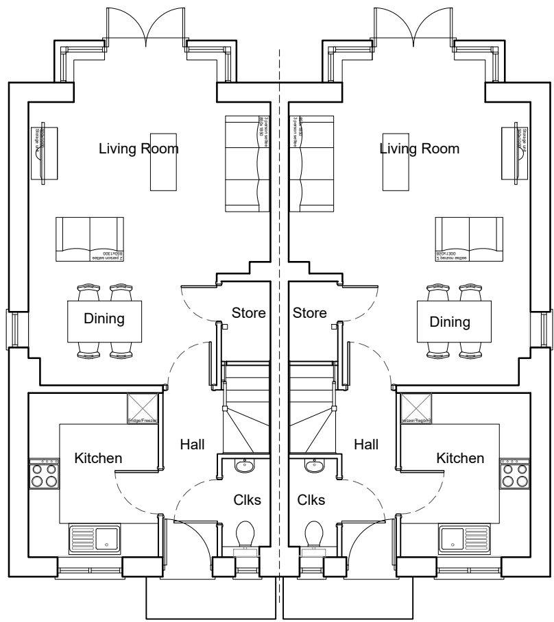
GROUND FLOOR
