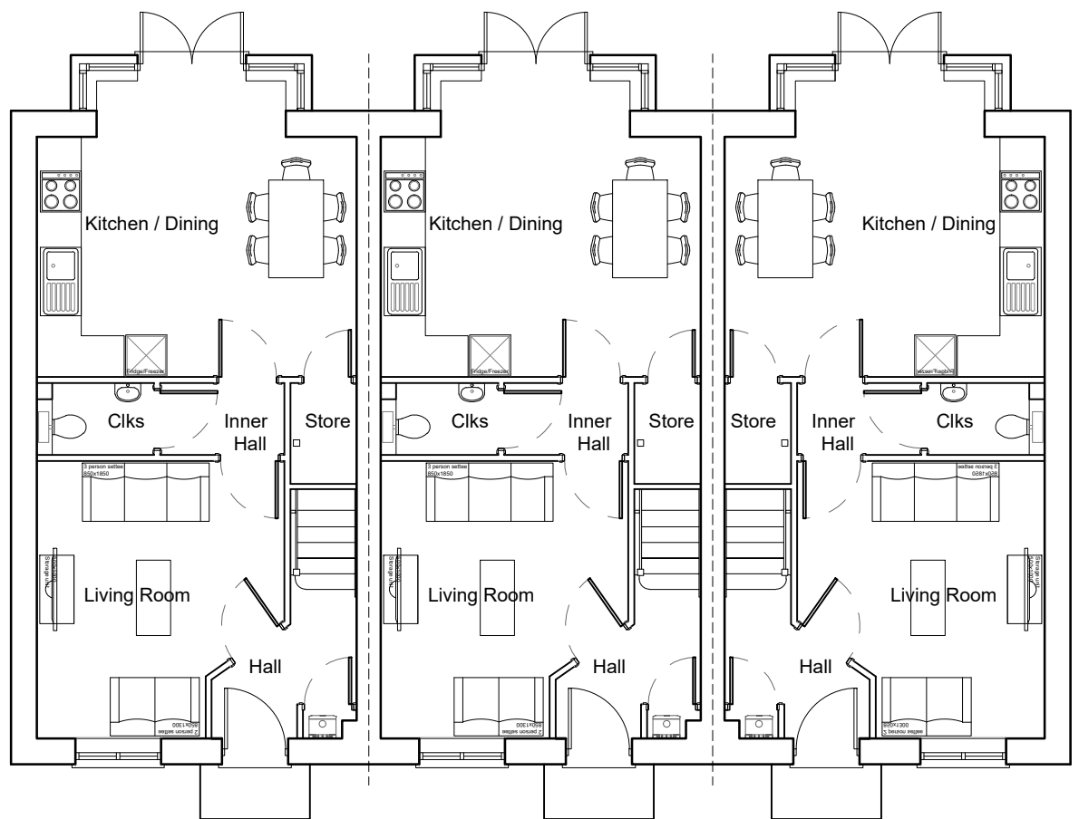
GROUND FLOOR
