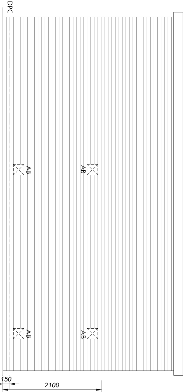
REAR ELEVATION BIN & CYCLE STORE BLOCK A2 PLOT 29-34
