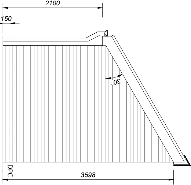
SIDE ELEVATION BIN & CYCLE STORE BLOCK A2 PLOT 29-34
