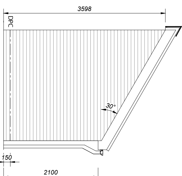
SIDE ELEVATION BIN & CYCLE STORE BLOCK A3 PLOT 58-63
