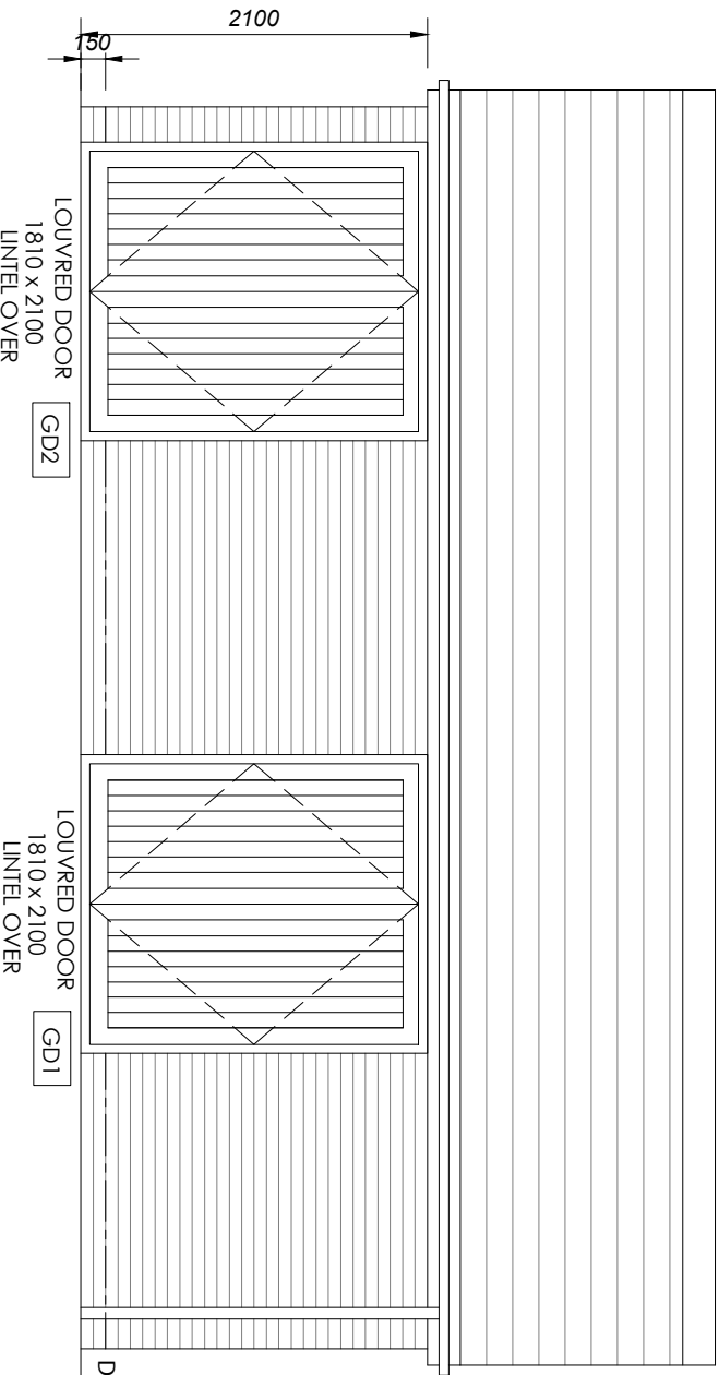
FRONT ELEVATION BIN & CYCLE STORE BLOCK A3 PLOT 58-63
