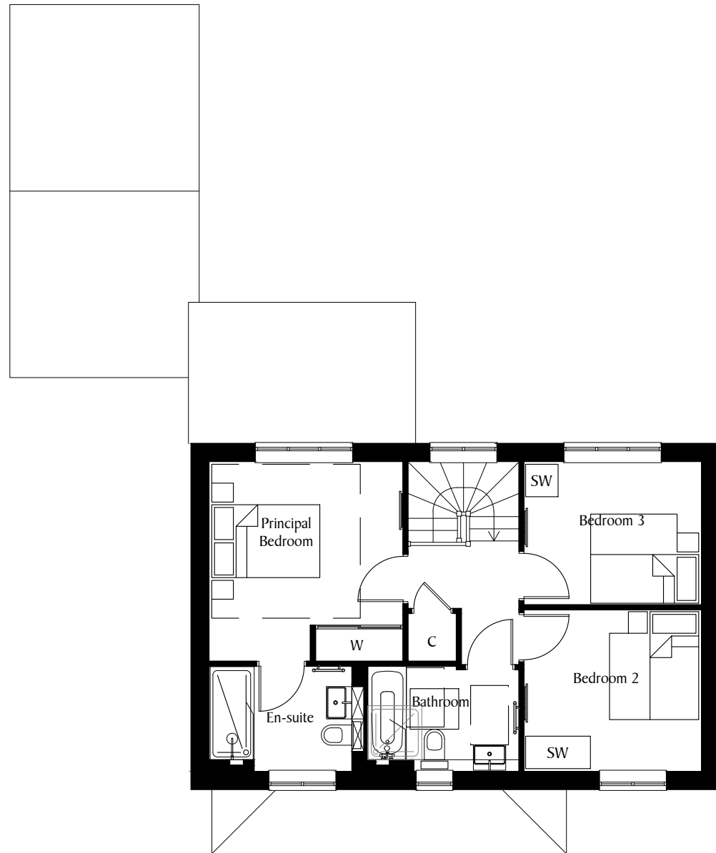
First Floor
