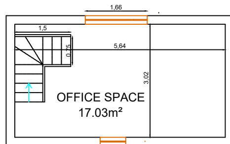
EXISTING 1ST FLOOR PLAN Scale 1: 100
