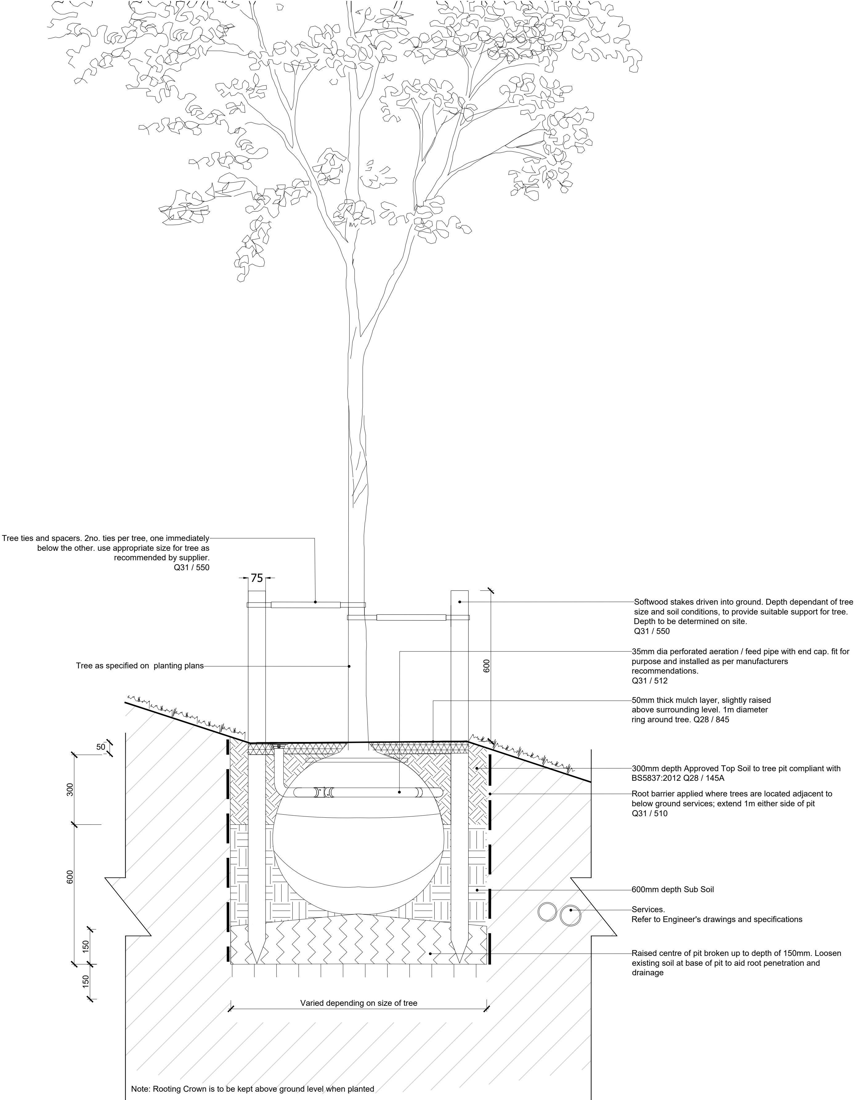
8701 2 Typical Detail - Tree planted in slope
