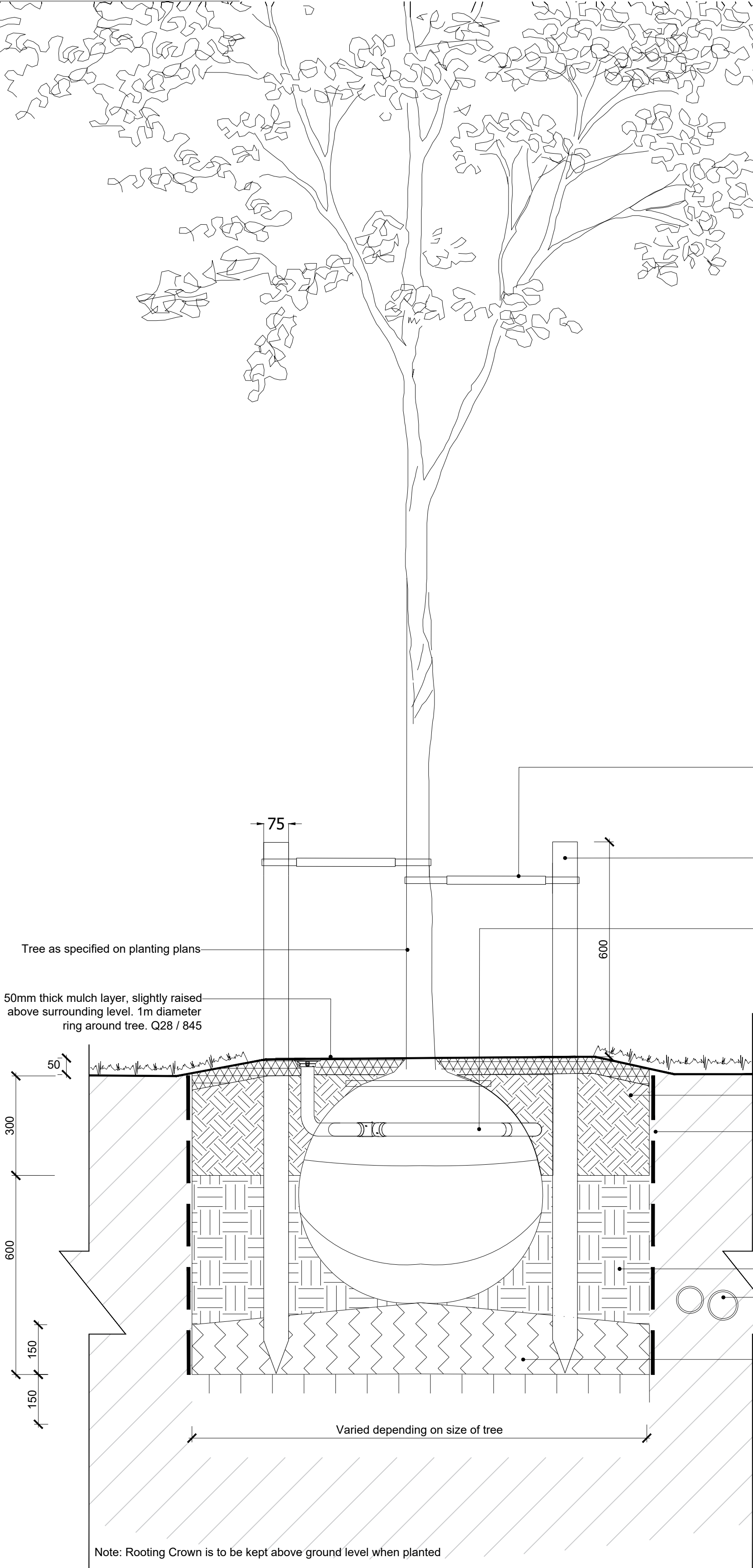
8701 1 Typical Detail - Tree with Double Staking
