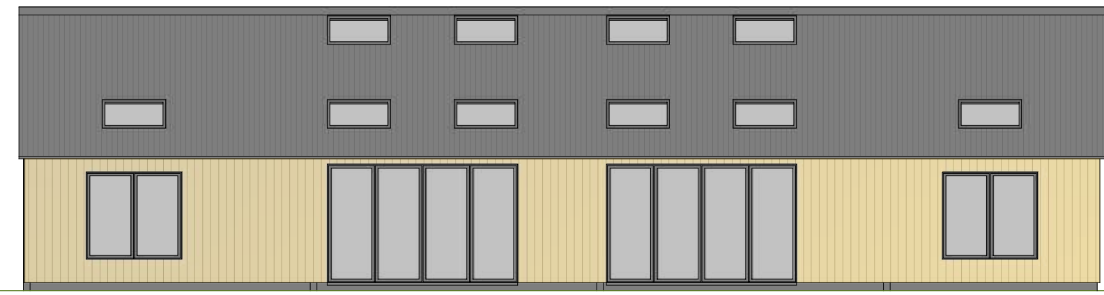
West Elevation 1:100
