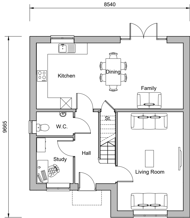
Ground Floor Plan Plot 194, 207 Plot 210 (handed)
