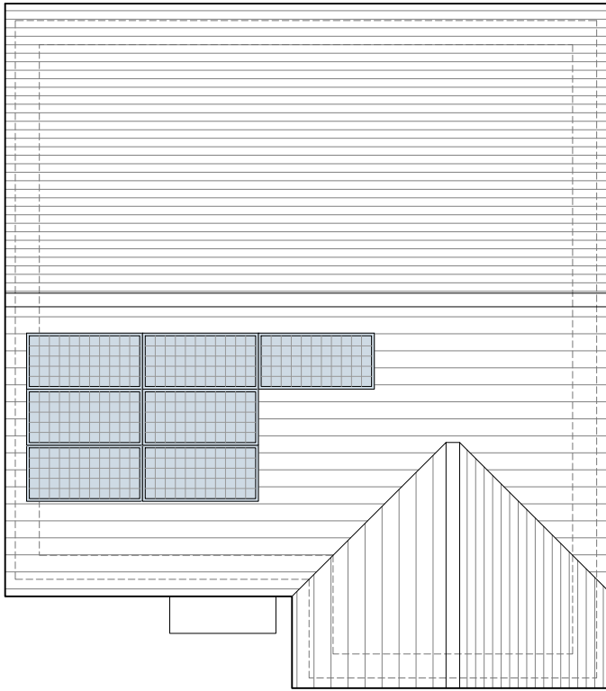
Roof Plan
