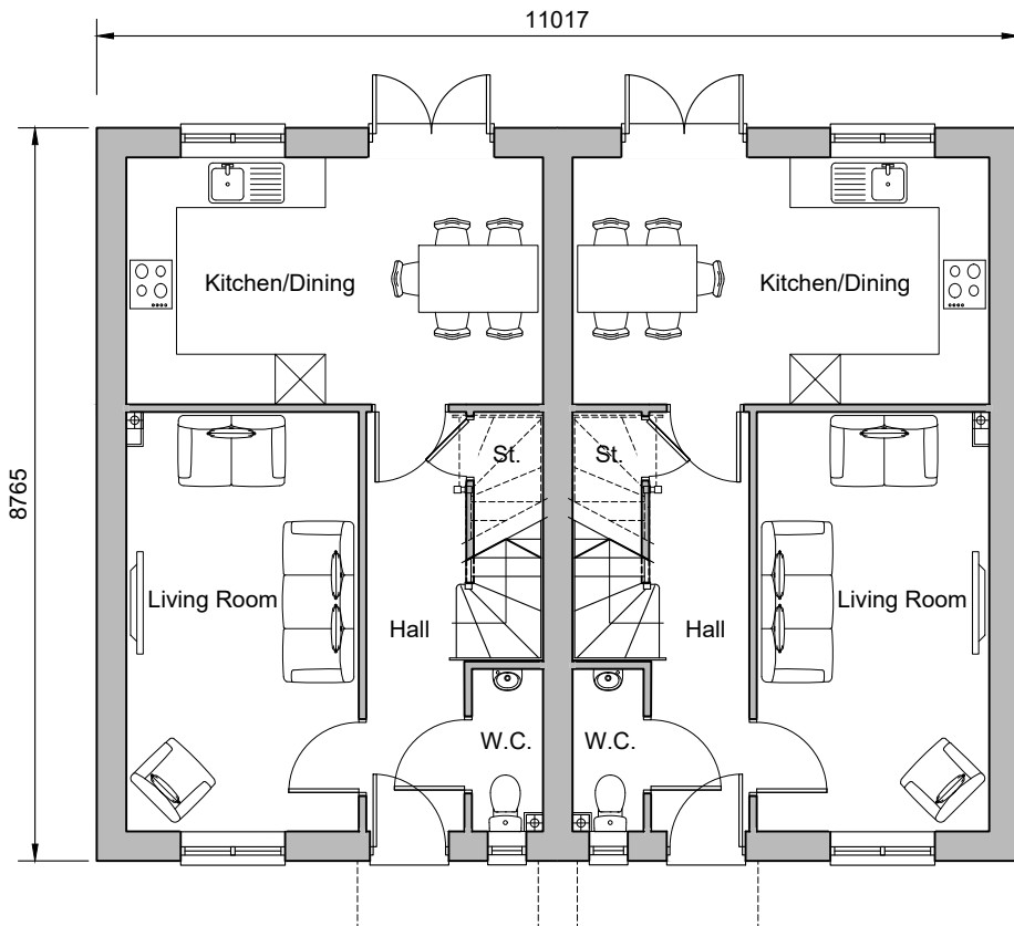
Ground Floor Plan Plots 195-196
