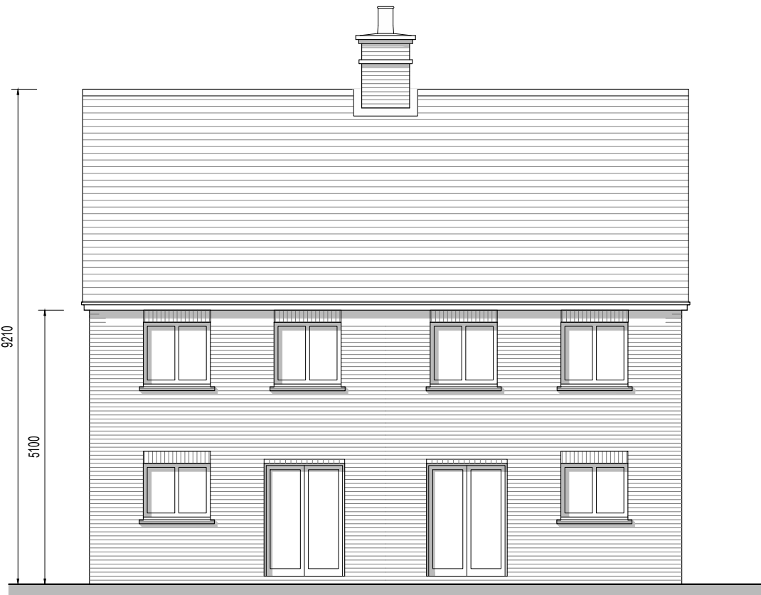
Rear Elevation
