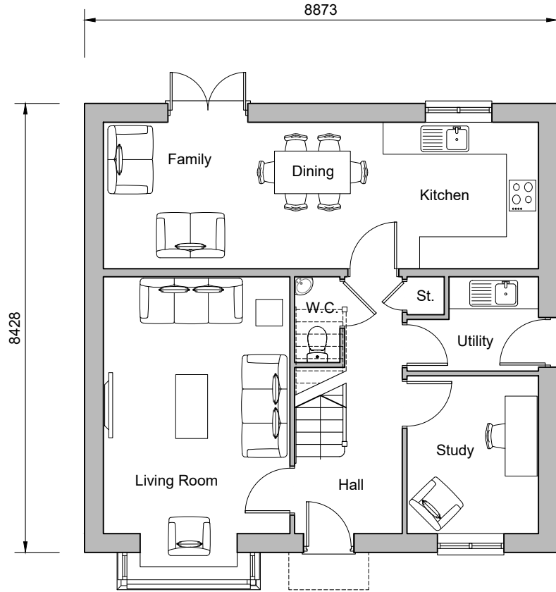
Ground Floor Plan Plot 208 Plots 198, 209 (handed)
