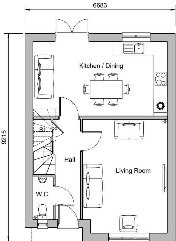
Ground Floor Plan Plot 249
