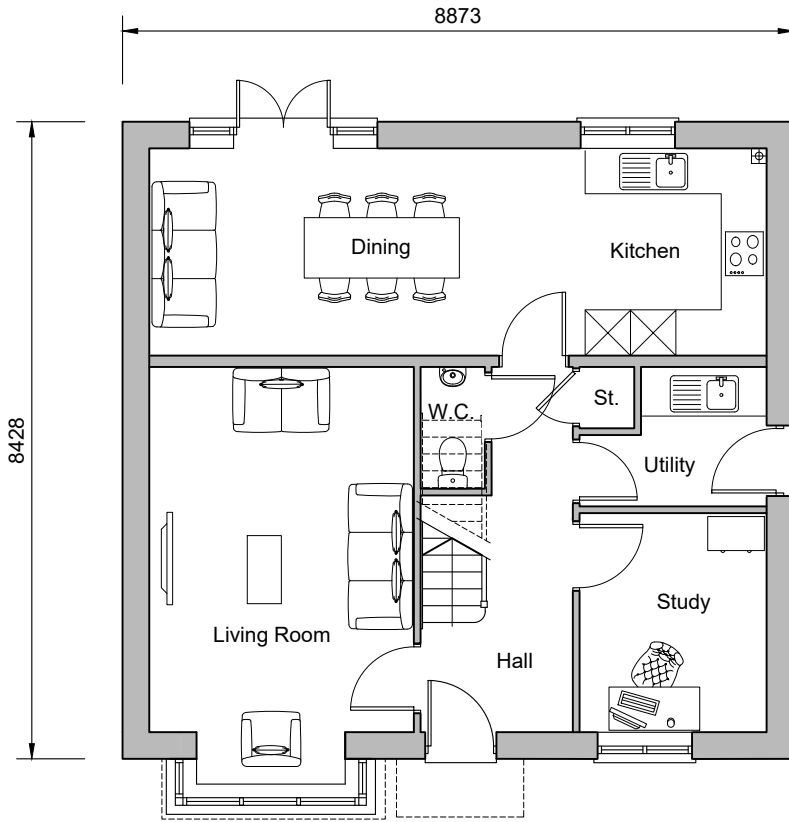
Ground Floor Plan Plot 205
