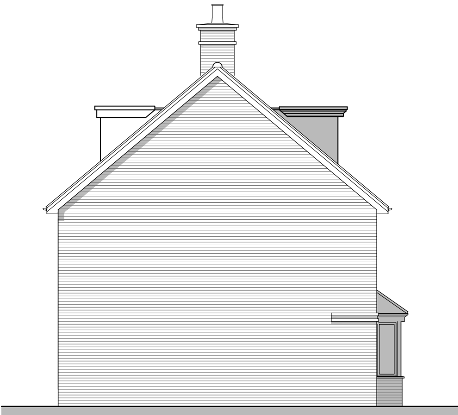
Side Elevation
