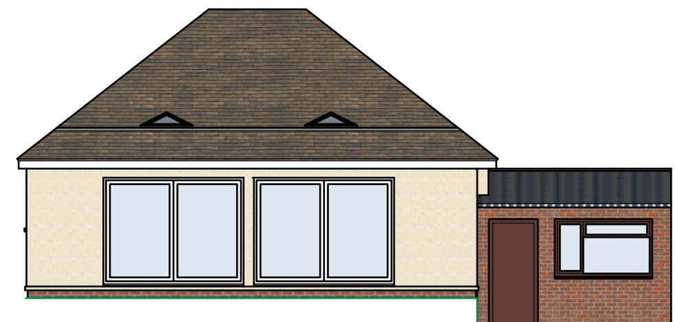
WEST ELEVATION
