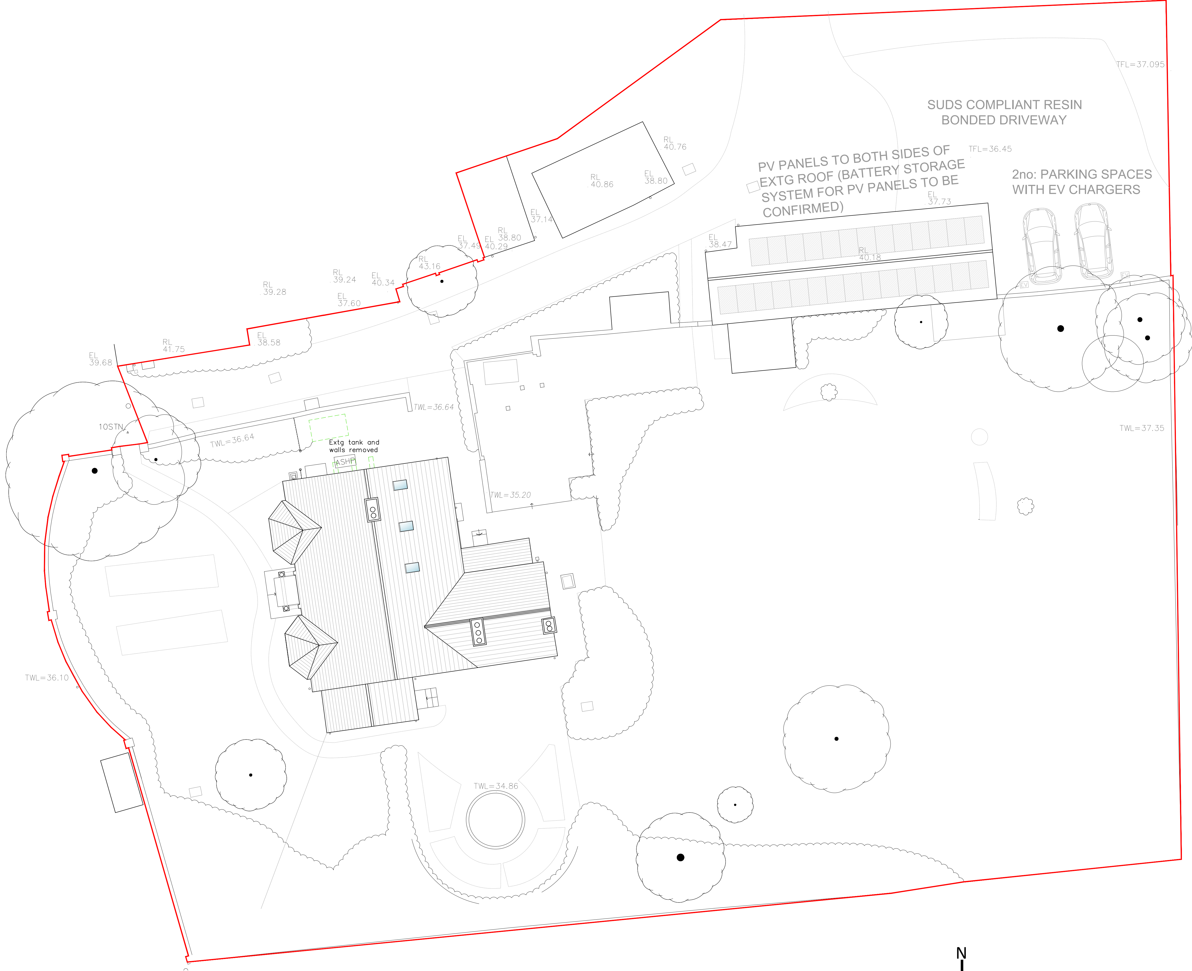
PROPOSED SITE LAYOUT 1:100
