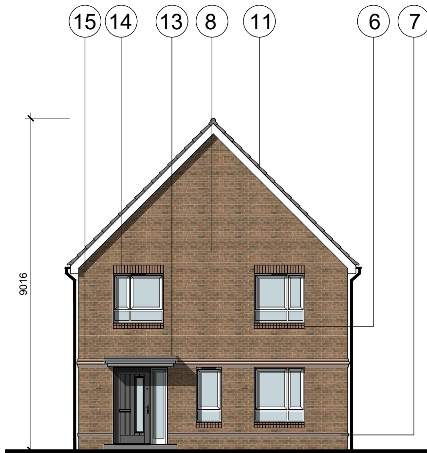
Front Elevation
