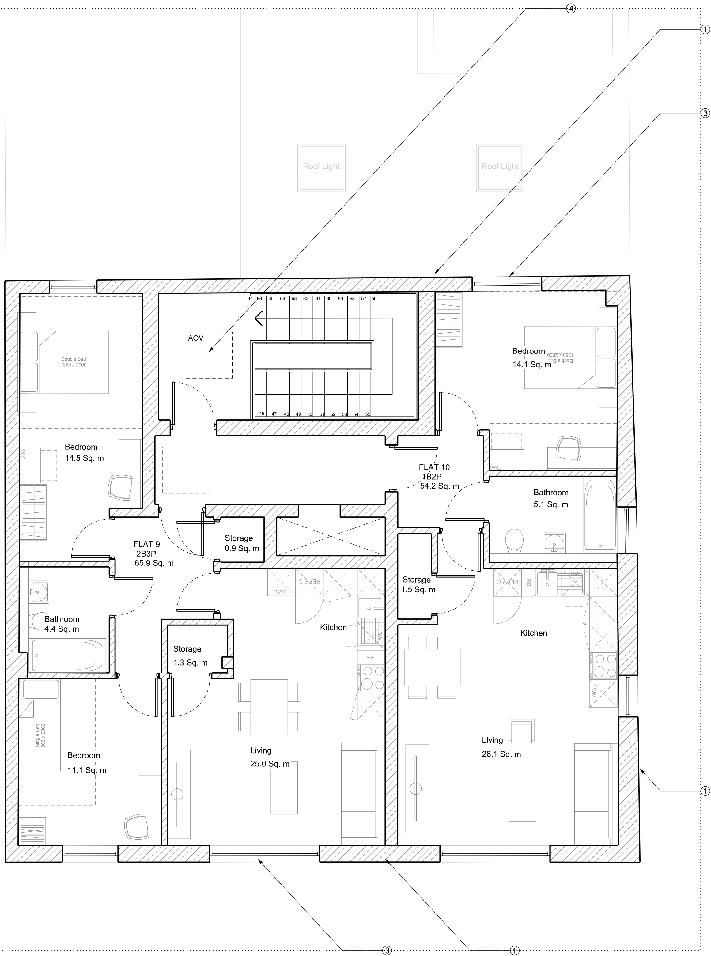
Proposed Third Floor Plan
