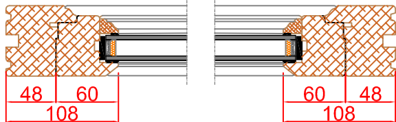
Section C-C
